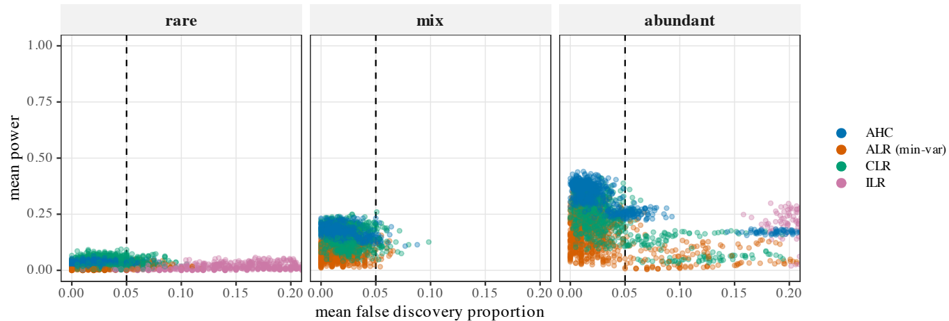
Power--FDP tradeoff across settings
