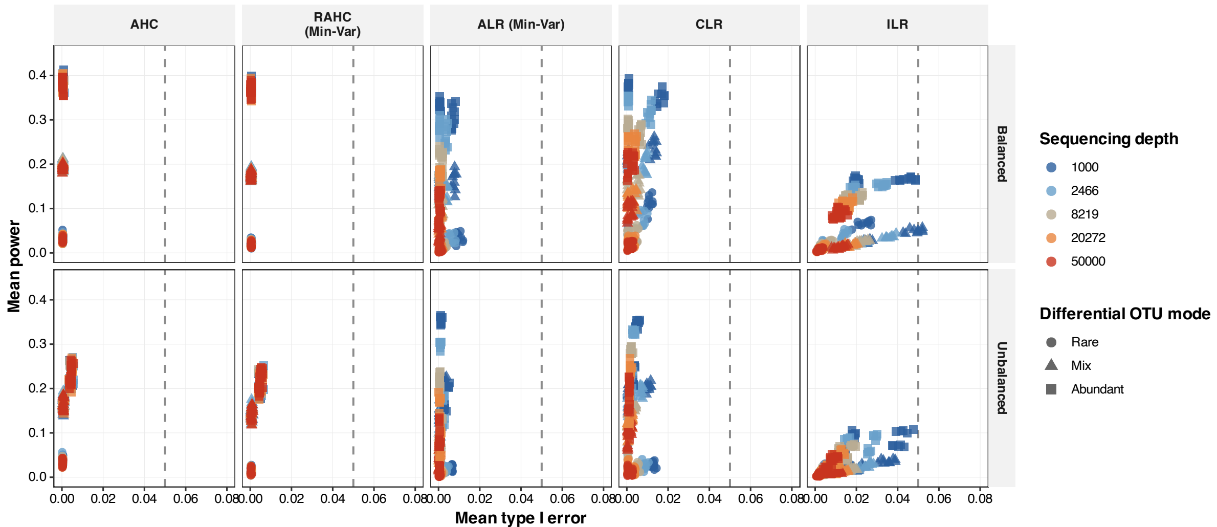
Power-type I error tradeoff: AHC vs logratio transformations
