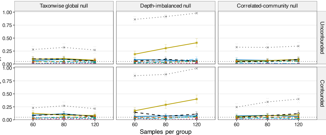
Family-wise Type I error
