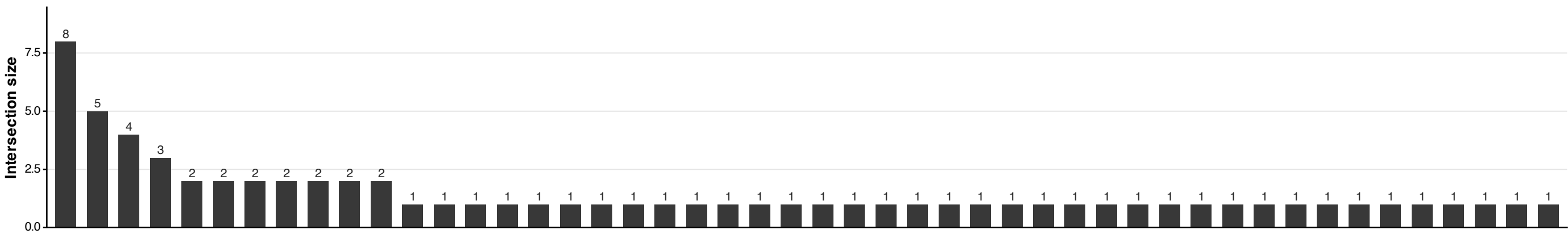
Significant-set intersections
