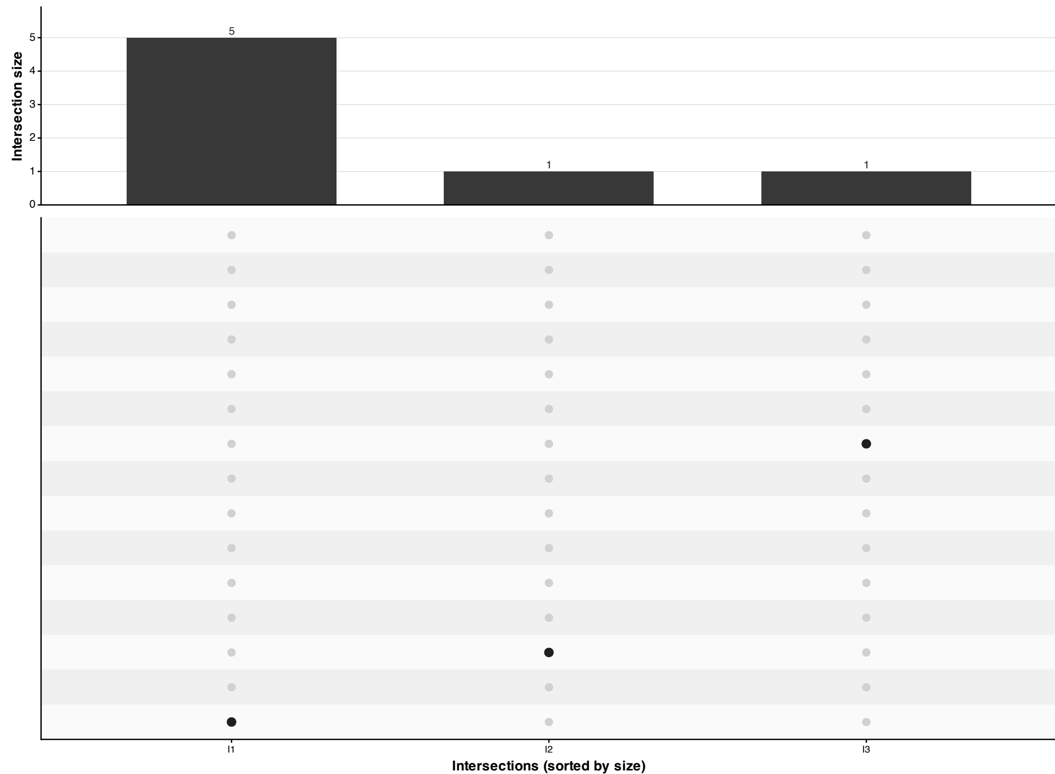
Significant-set intersections
