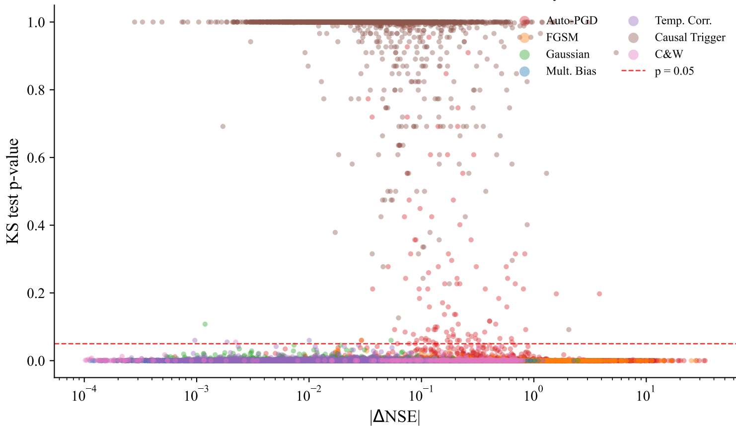
Attack Effectiveness vs. Statistical Detectability
