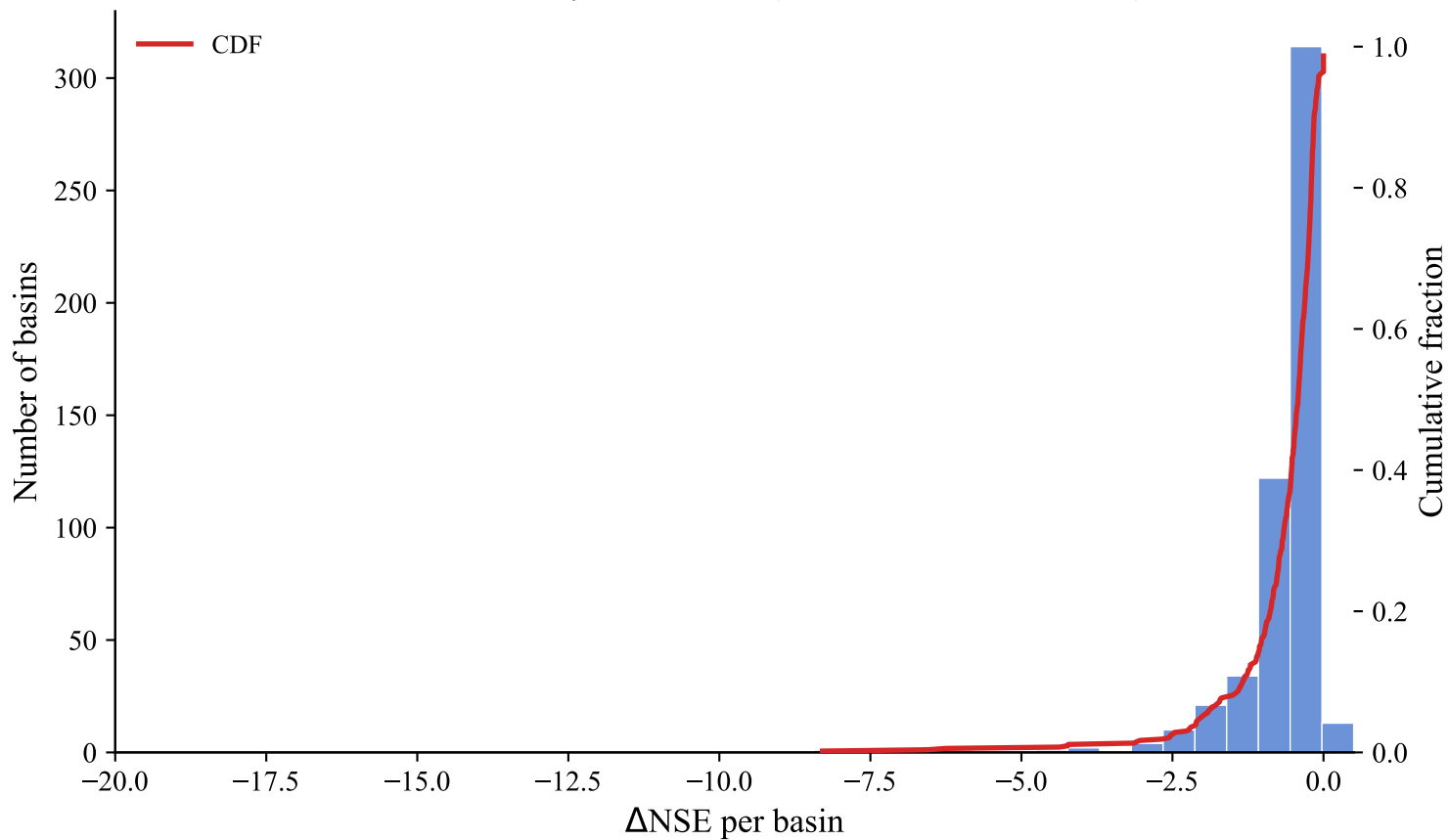
Basin Vulnerability Distribution (Auto-PGD, \epsilon=0.1 , N=531)
