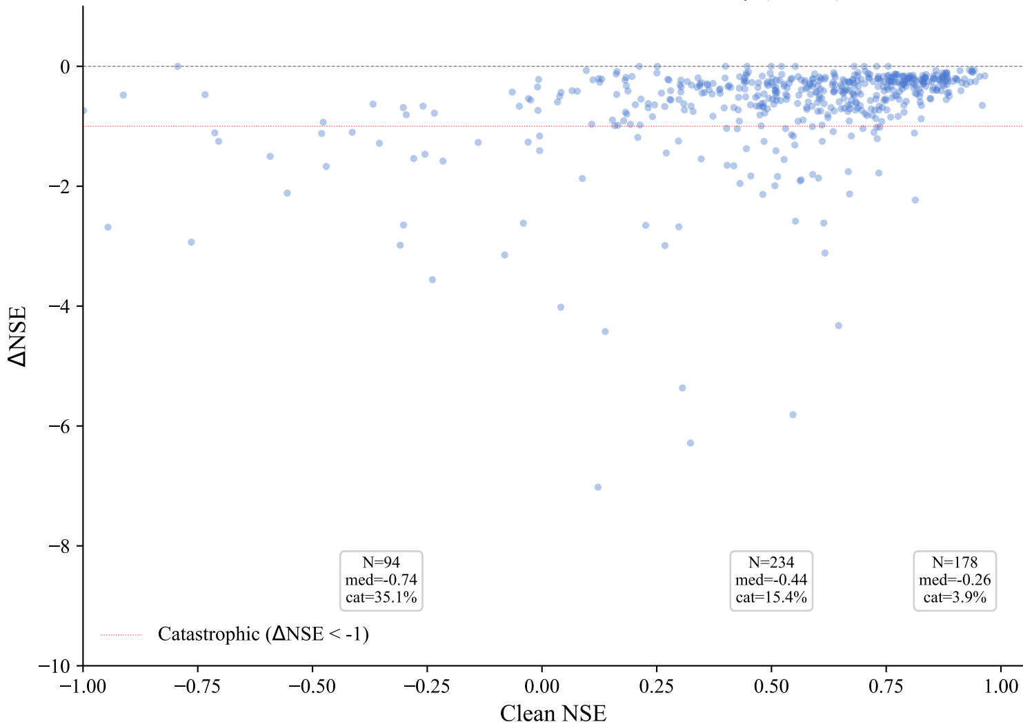
Baseline Performance vs. Adversarial Vulnerability (N=524)
