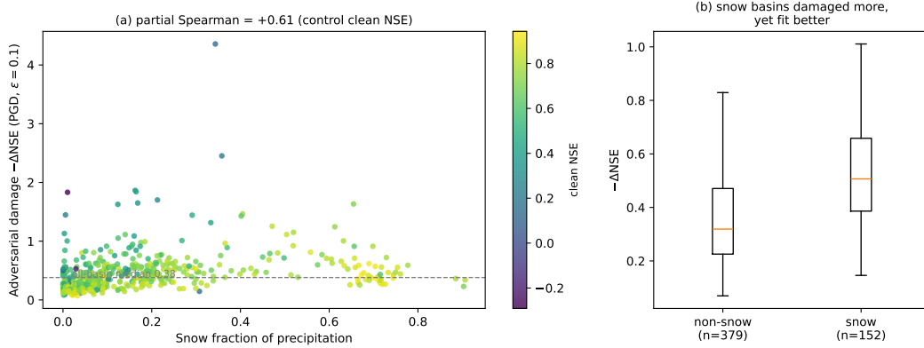
Figure 3 — Adversarial damage ( -\Delta\text{NSE} , scheduled-step PGD, \varepsilon = 0.1 ) versus snow fraction across the 531 basins. (a) Per-basin damage rises with snow fraction; points colored by clean NSE, dashed line at the all-basin median. Partial Spearman \rho = 0.61 after controlling for clean NSE. (b) Snow-dominated catchments (snow fraction above 0.2) are damaged more than the rest, despite being fit better on clean data.
