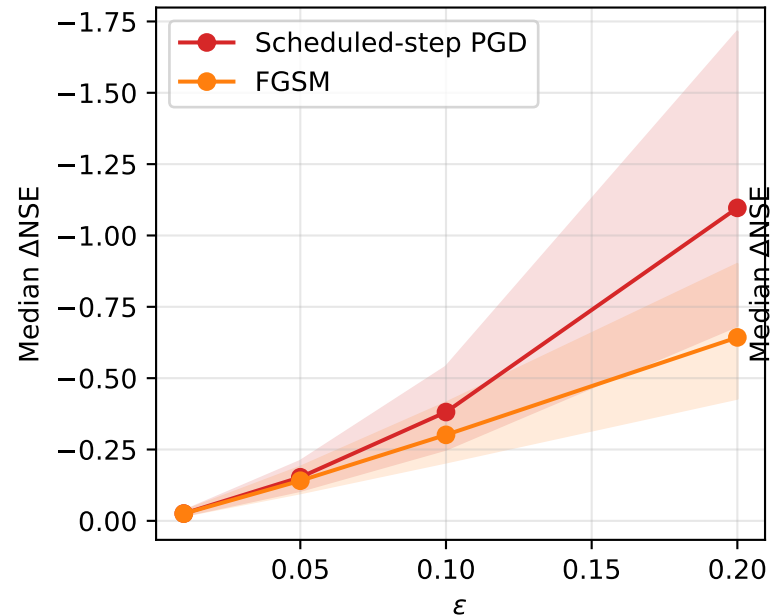
(a) Gradient attacks
