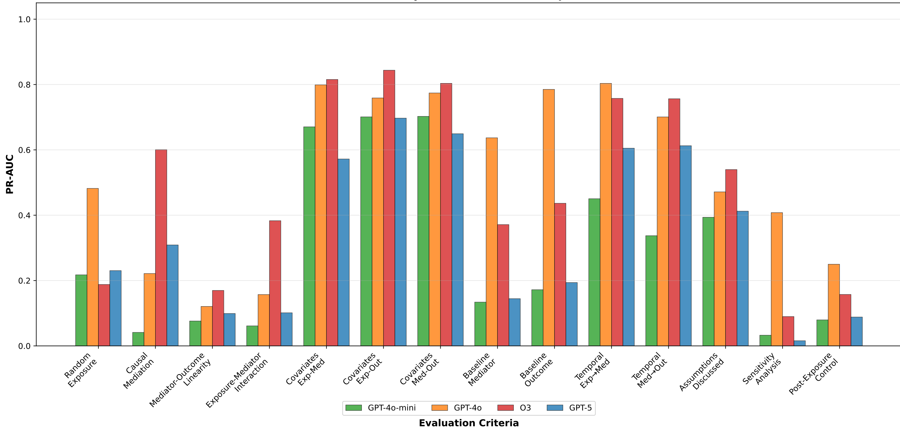
PR-AUC by Criterion (Basic Prompts)
