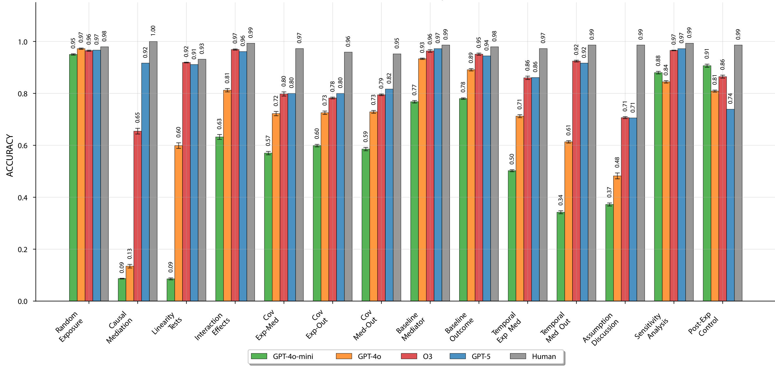
ACCURACY for Basic Prompts
