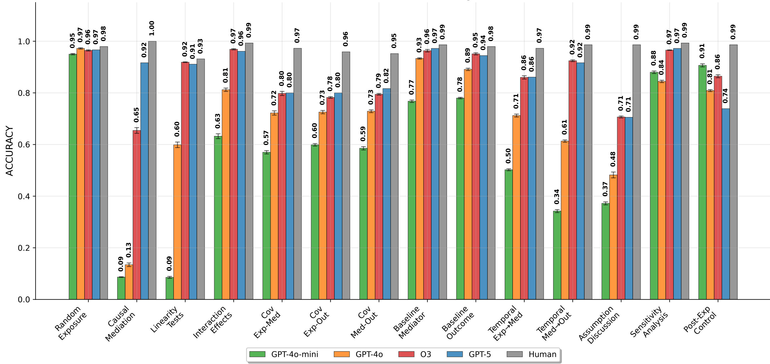
ACCURACY - Basic Prompts
