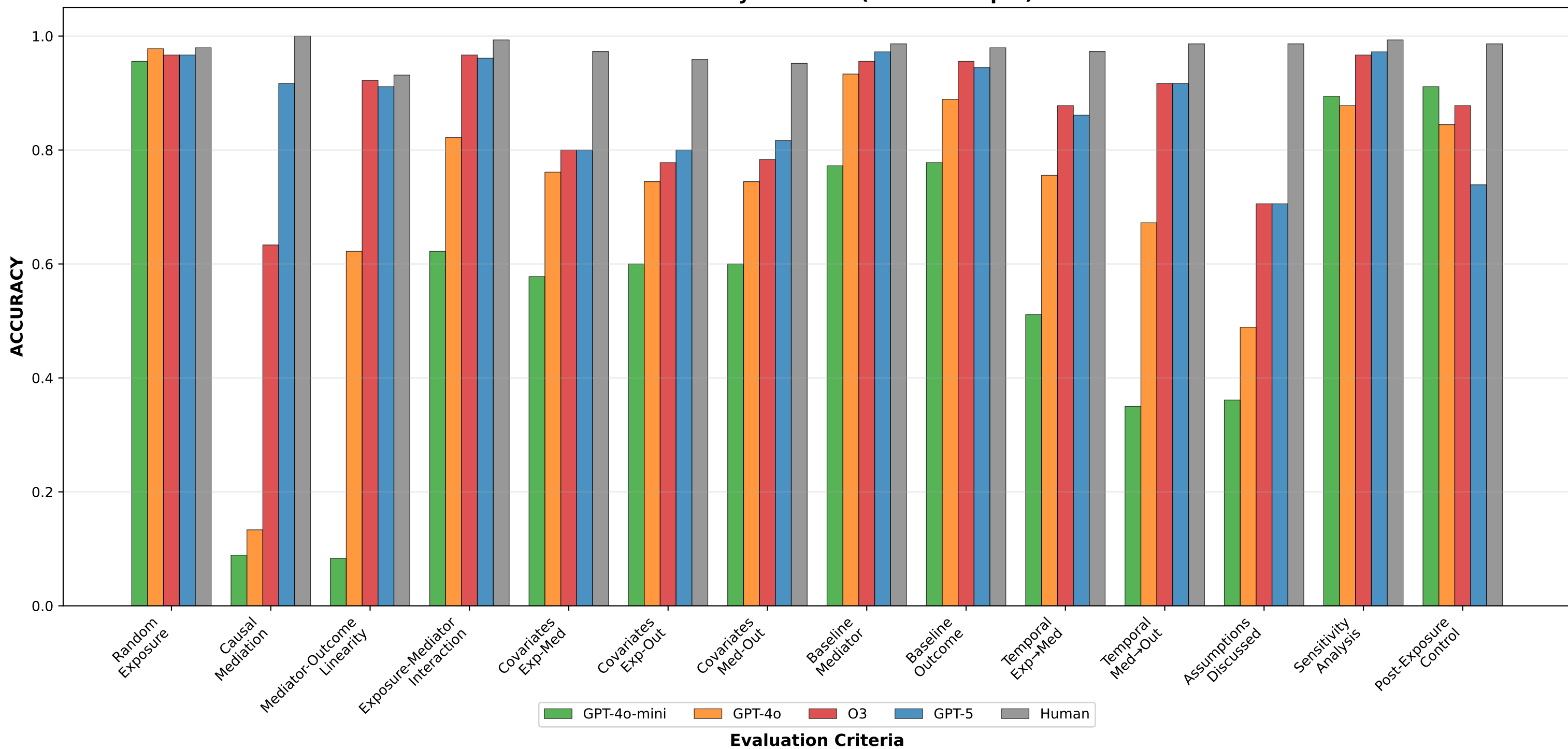
ACCURACY by Criterion (Basic Prompts)
