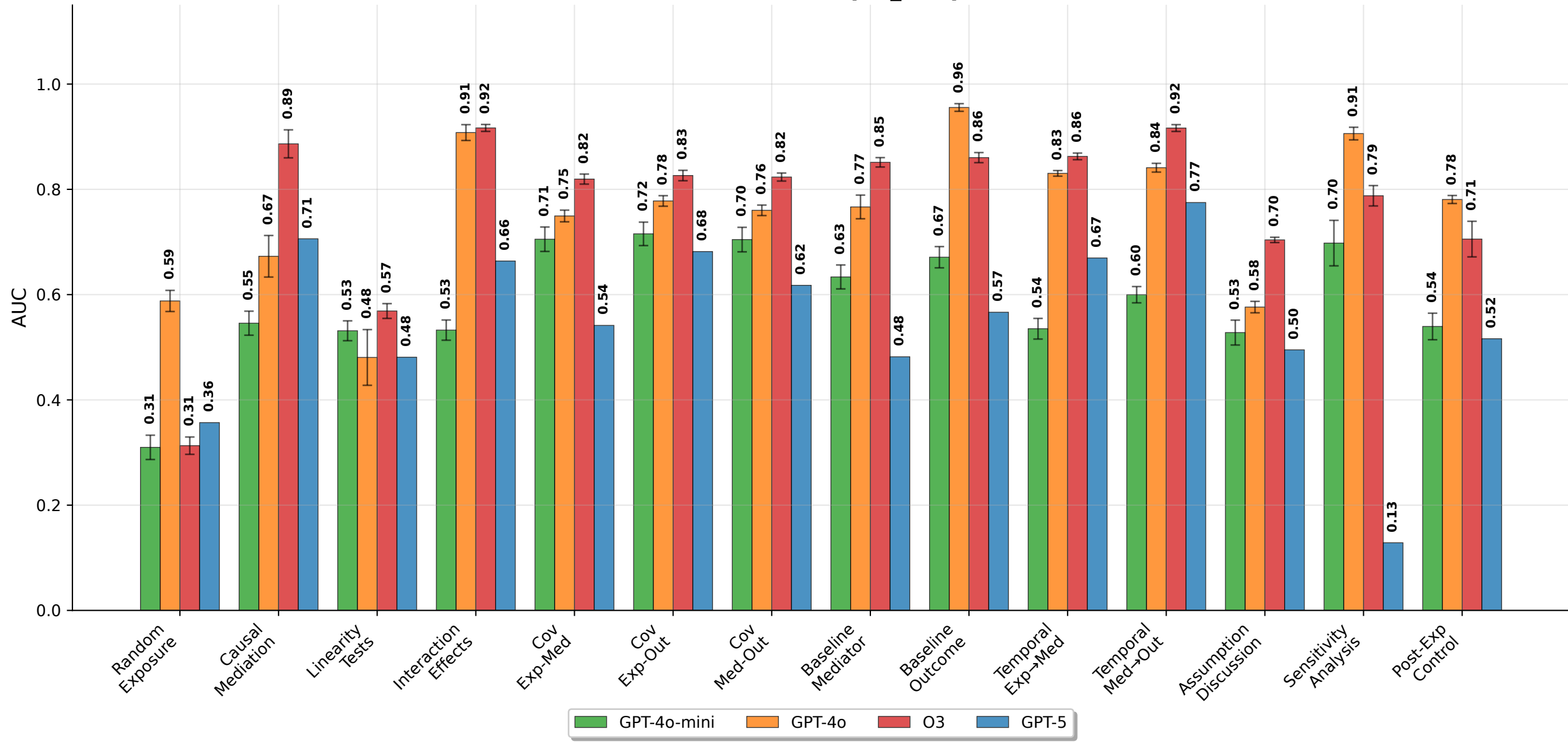
AUC - Basic Prompts_temp1.0
