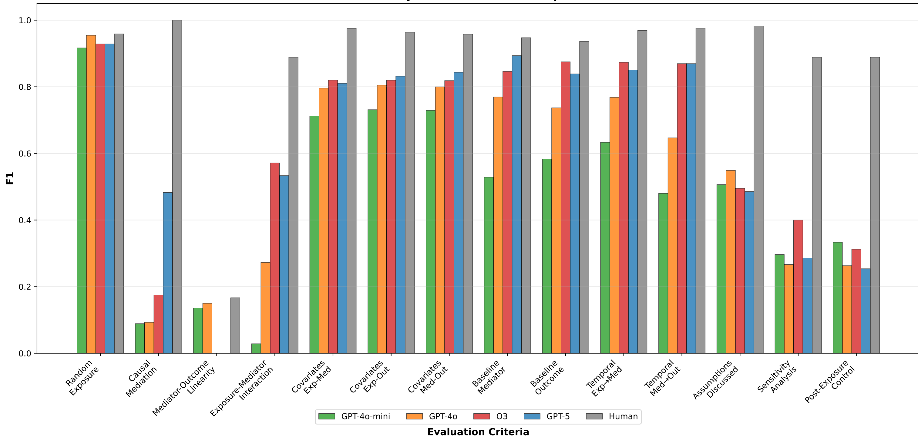
F1 by Criterion (Basic Prompts)
