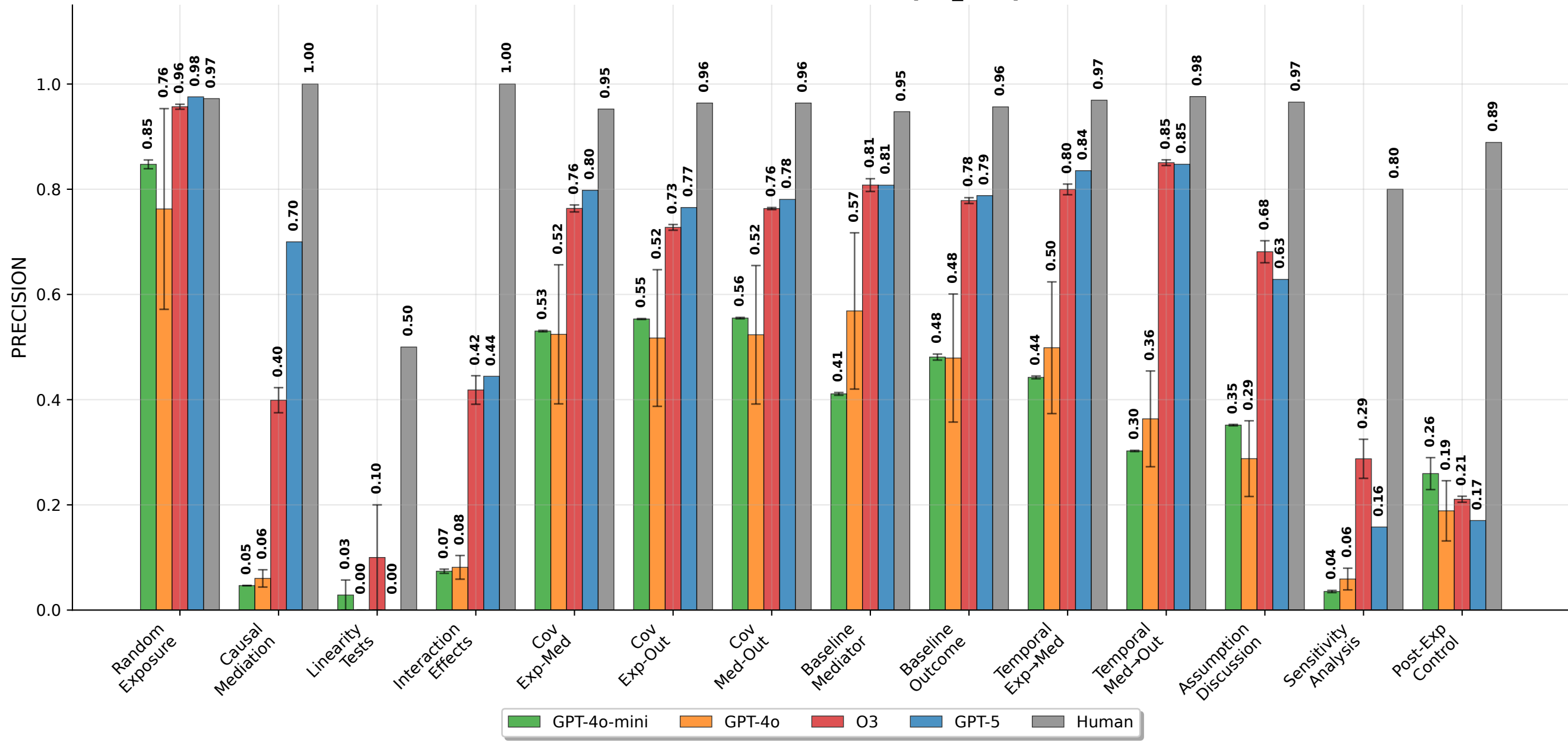
PRECISION - Detailed Prompts_temp1.0
