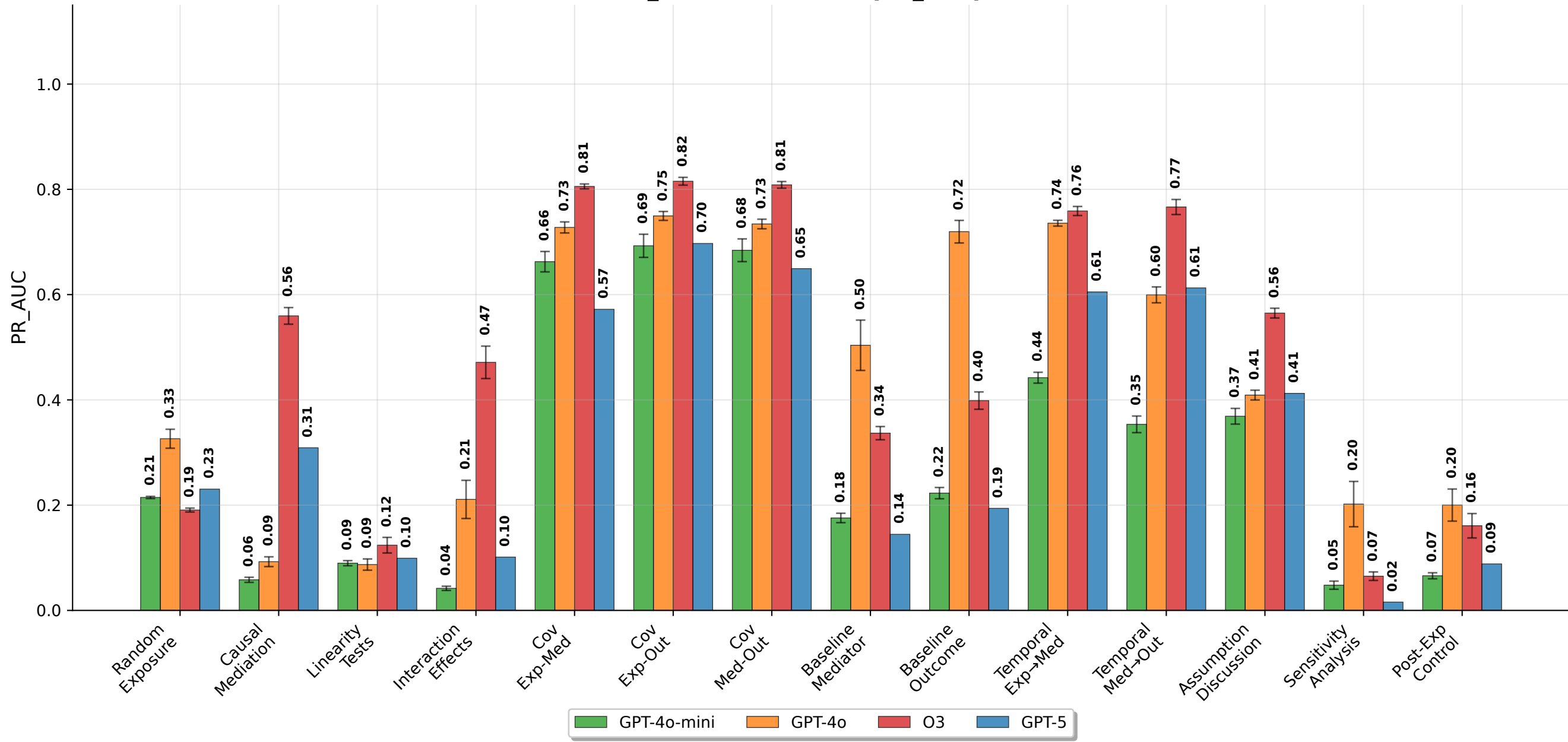
PR_AUC - Basic Prompts_temp1.0
