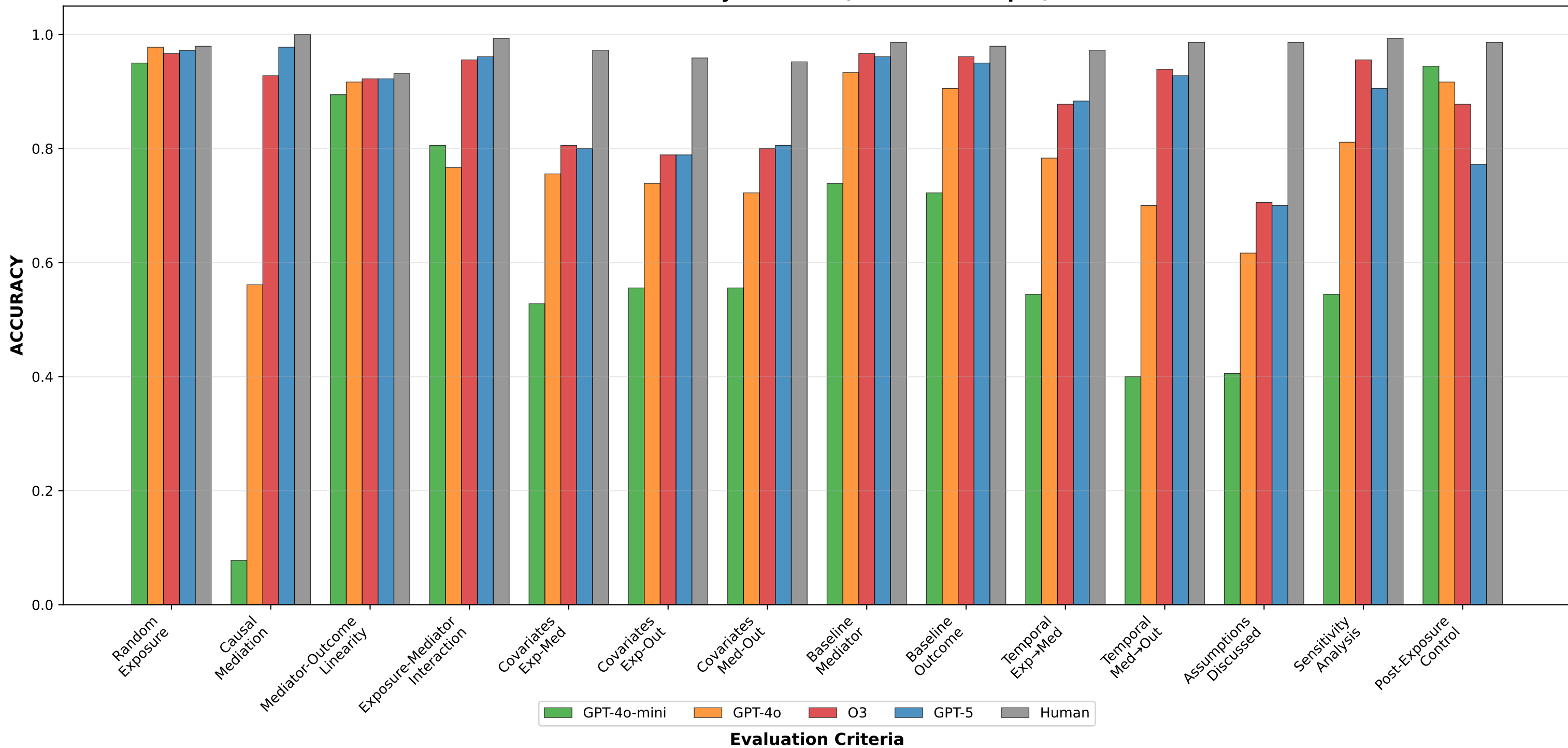
ACCURACY by Criterion (Detailed Prompts)
