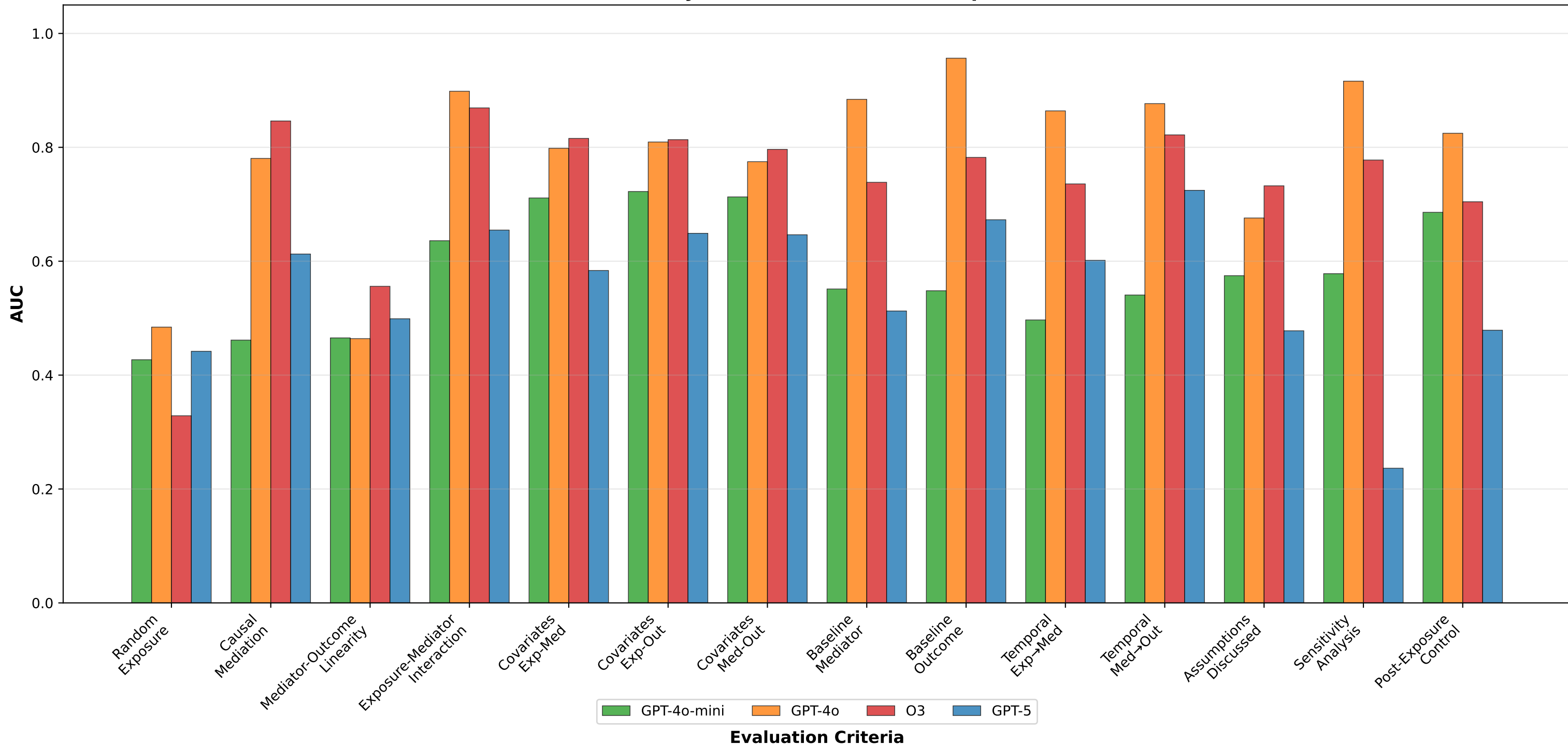
AUC by Criterion (Detailed Prompts)
