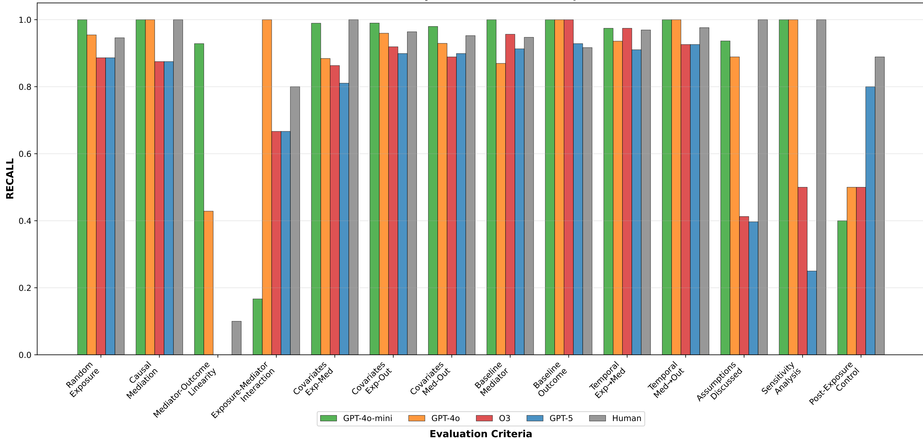
RECALL by Criterion (Basic Prompts)
