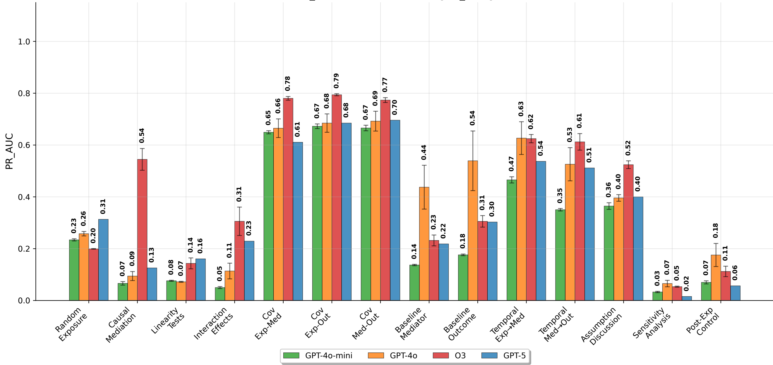
PR_AUC - Detailed Prompts_temp1.0
