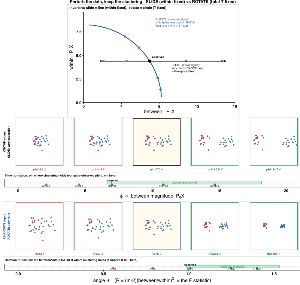
Figure 2: The contrast plane ( \|\mathbf{P}_0\mathbf{X}\|_F, \|\mathbf{P}_1\mathbf{X}\|_F ). The known- \sigma tests fix the within-cluster scatter and vary the separation ( \rightarrow \chi ); the studentized test (Section 4) fixes the total T and varies the ratio R ( \rightarrow F ). Source: sims/plot_decomposition.R .
