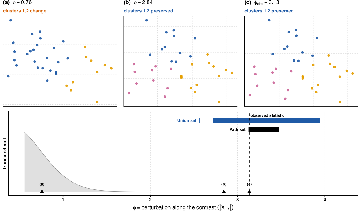
Figure 3: Condition on less \Rightarrow more power, on one dataset ( p_{\text{path}} = 0.83 , p_{\text{union}} = 5 \times 10^{-4} ). Top: the data perturbed along the contrast, \mathbf{x}'(\phi) . (a) far below the conditioning set the two tested clusters merge (recoloured); (b) at a smaller separation inside the union set — but outside the path interval — they are still recovered; (c) the observed data. Bottom: the set of \phi preserving the two clusters. The path test conditions on the single interval at the observed statistic (dashed); the union test on the whole set, which extends below it. Truncated- \chi null underneath. Source: sims/plot_conditioning_set.R .
