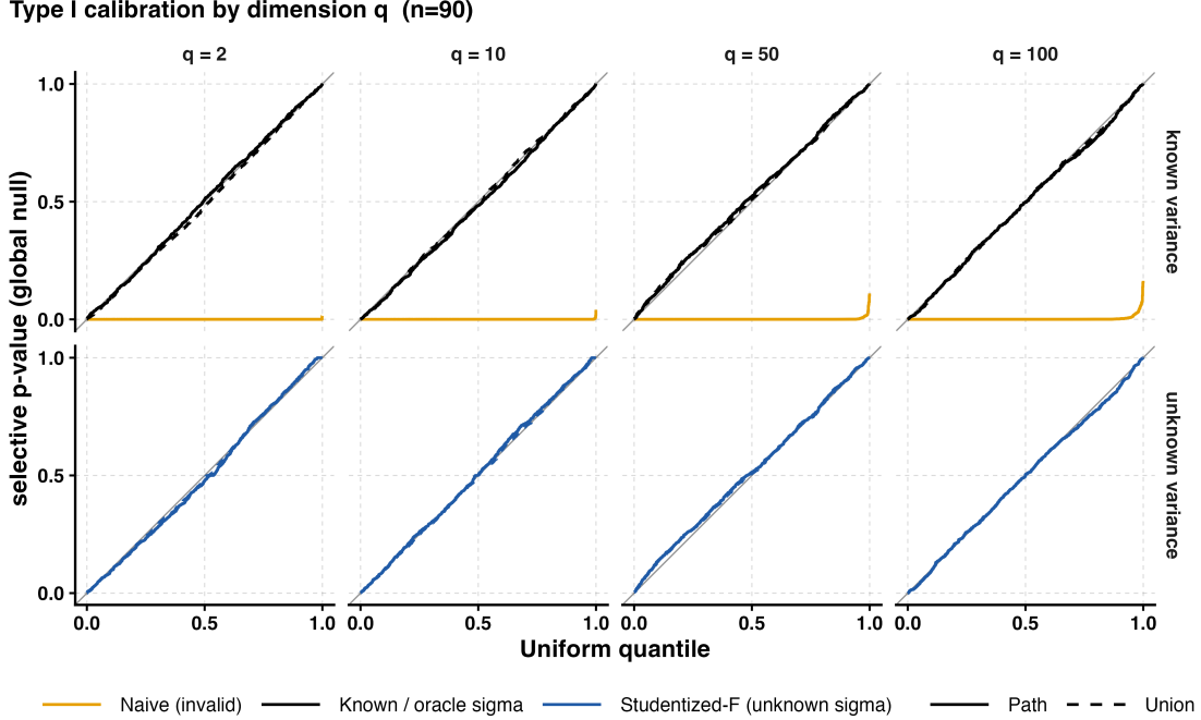
Figure 4: Selective Type I error ( n = 90 , K = 3 ). QQ-plots of the null p -values against Uniform(0, 1), faceted by dimension q . Top: known- \sigma tests; bottom: studentized tests. The selective path (solid) and union (dashed) lie on the 45° line at every q , while the naive p -value (orange) collapses below it. Source: sims/plot_cw_typeI.R .
