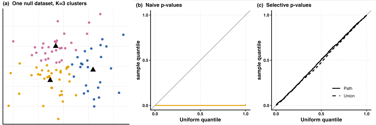
Figure 1: The double-dipping problem. (a) One null dataset ( \mu = \mathbf{0} ); k -means with K = 3 nonetheless returns three clusters (centroids as triangles). (b) QQ-plot of the naive p -values for the cluster-mean differences over many such null datasets: they collapse far below the 45^\circ line — grossly anti-conservative. (c) The selective path and union p -values are uniform, controlling the selective Type I error. Source: sims/plot_intro_motivation.R .
