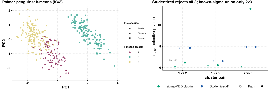
Figure 7: Palmer penguins, K = 3 (Table 1). Left: the four standardized features in the first two PCs, true species as point shape and k -means clusters as colour. Right: the selective p -value ( -\log_{10} ) for each cluster pair, by method. Source: penguins.png .
