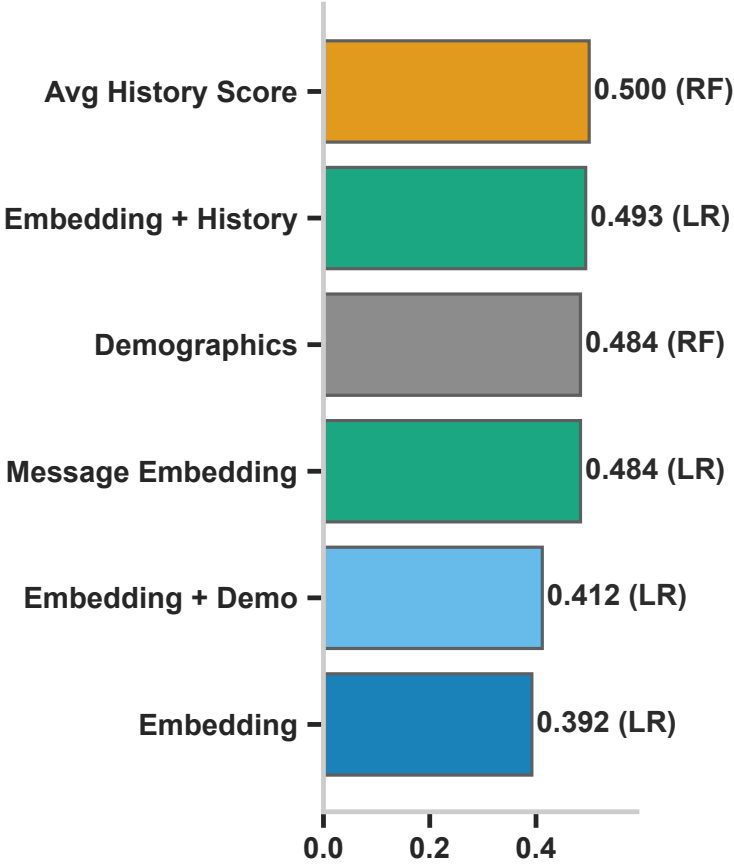
Content | Accuracy
