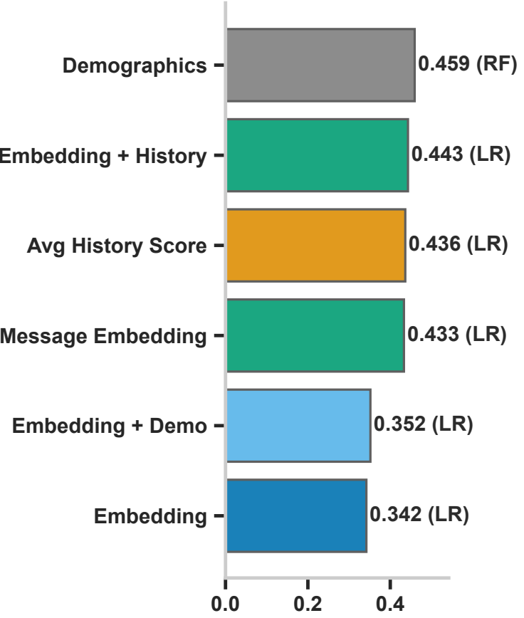
Coping | Accuracy
