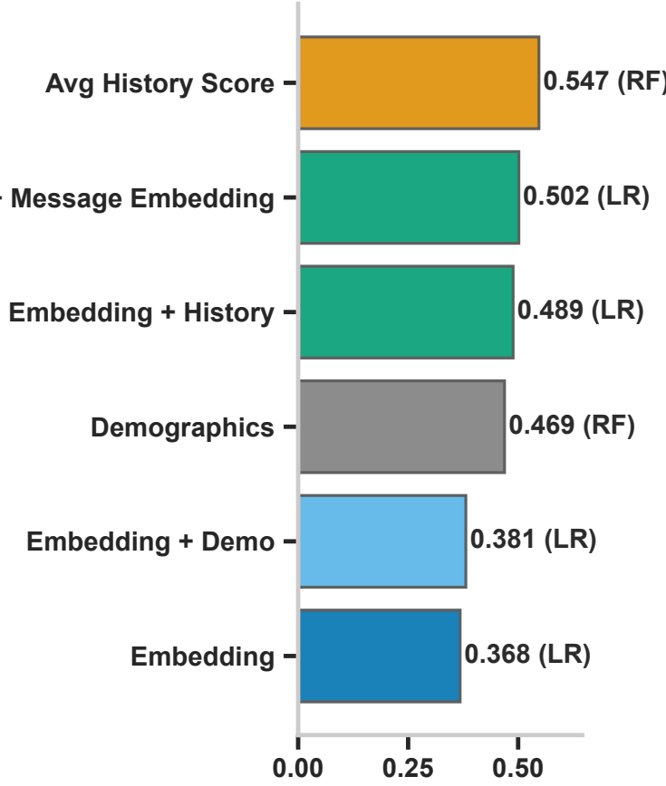
Quitting | Accuracy
