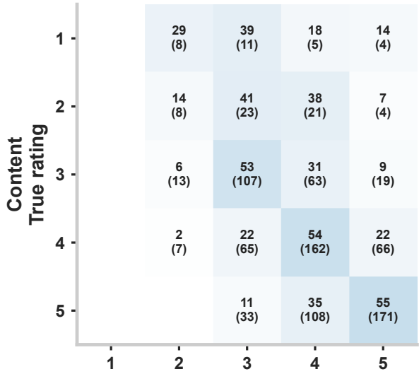
QWK=0.554 Acc=0.420
