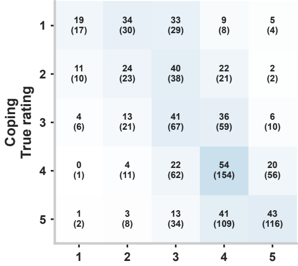
QWK=0.617 Acc=0.420
