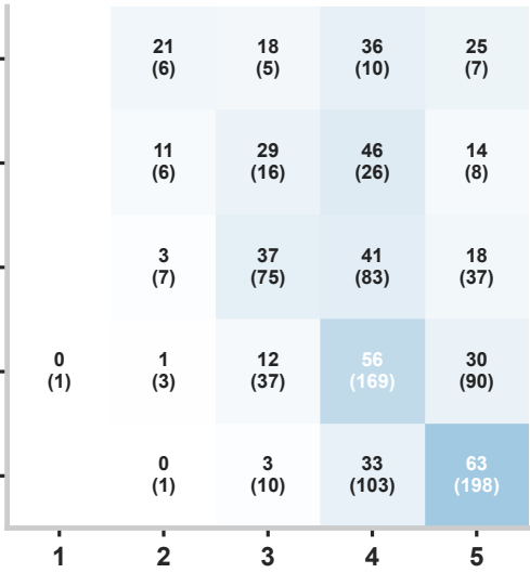
QWK=0.503 Acc=0.431
