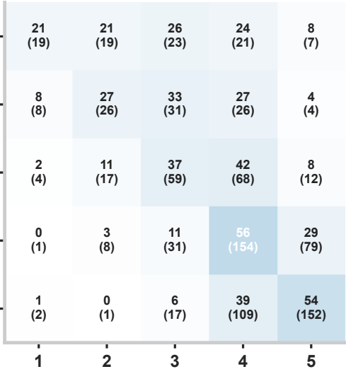
QWK=0.559 Acc=0.457
