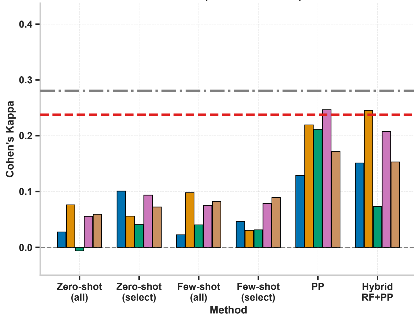
Content (common N=298)
