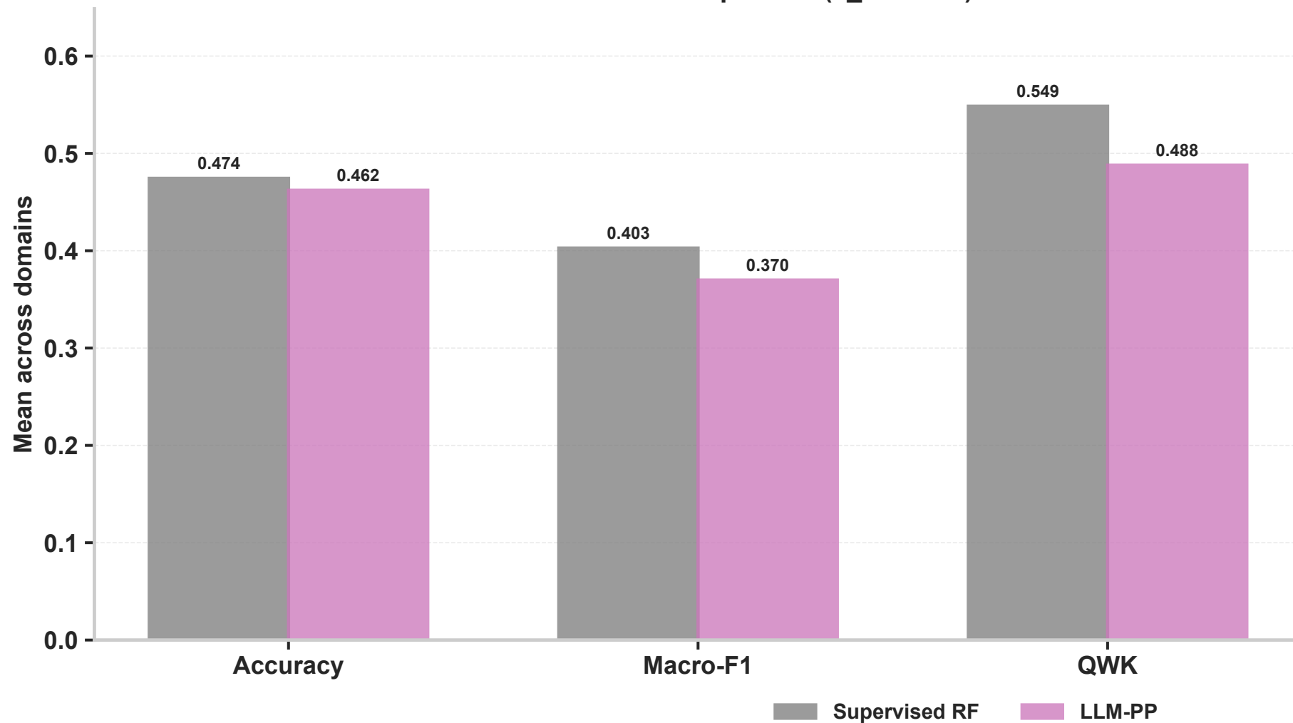
Strict fixed-feature comparison (k_train = 7)
