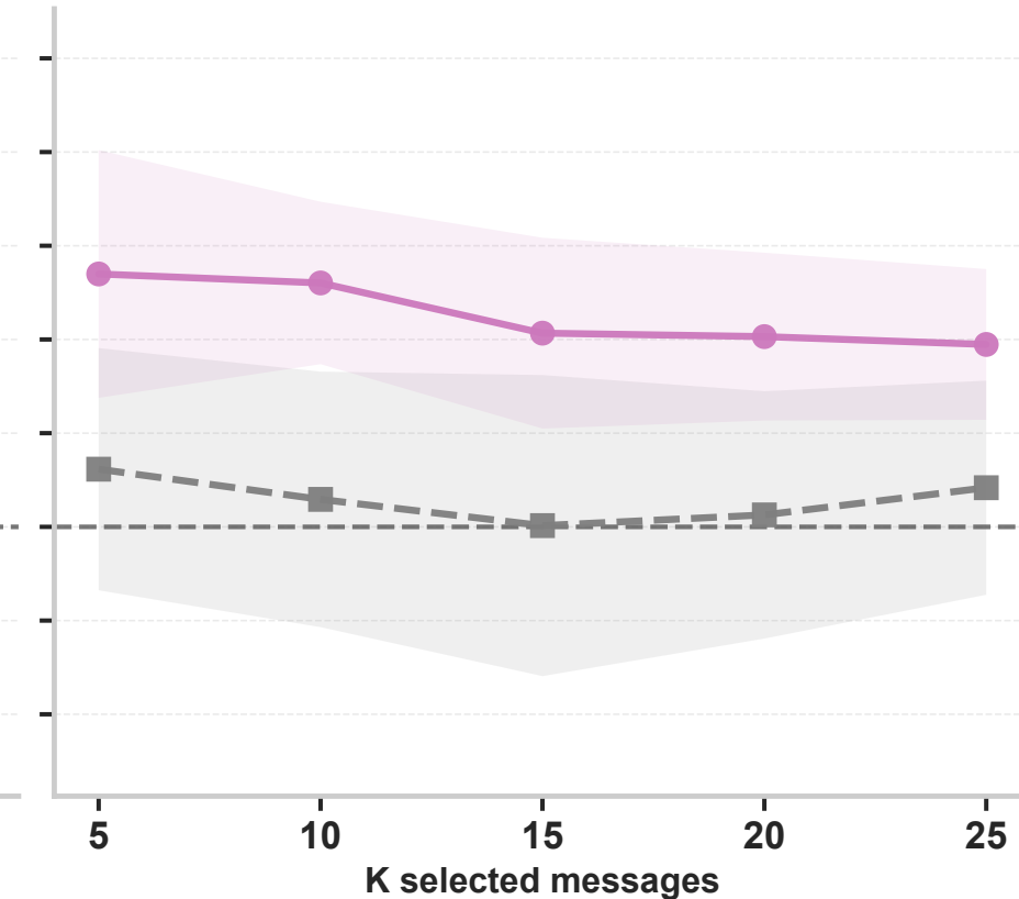
Message-selection gain over random with demographics + history + message embedding (95% CI bands, k_train = 7)
