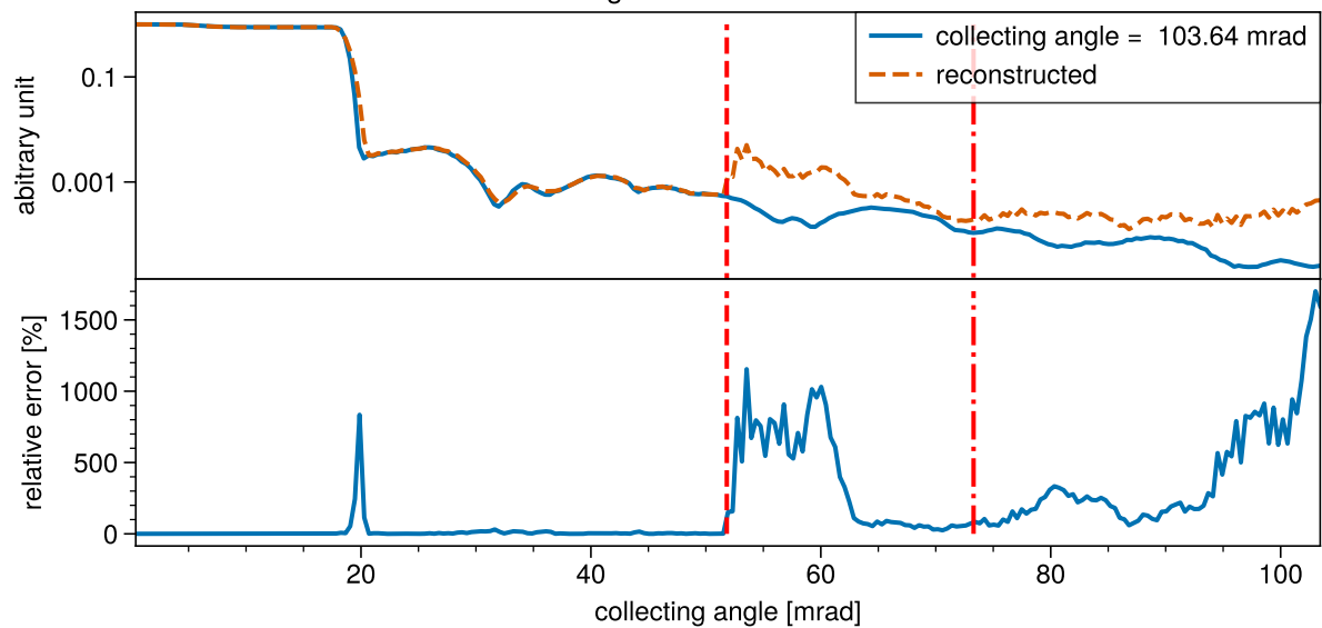
Radial Averaged Count of Diffraction Pattern
