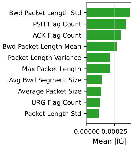
C. Top attributed features
