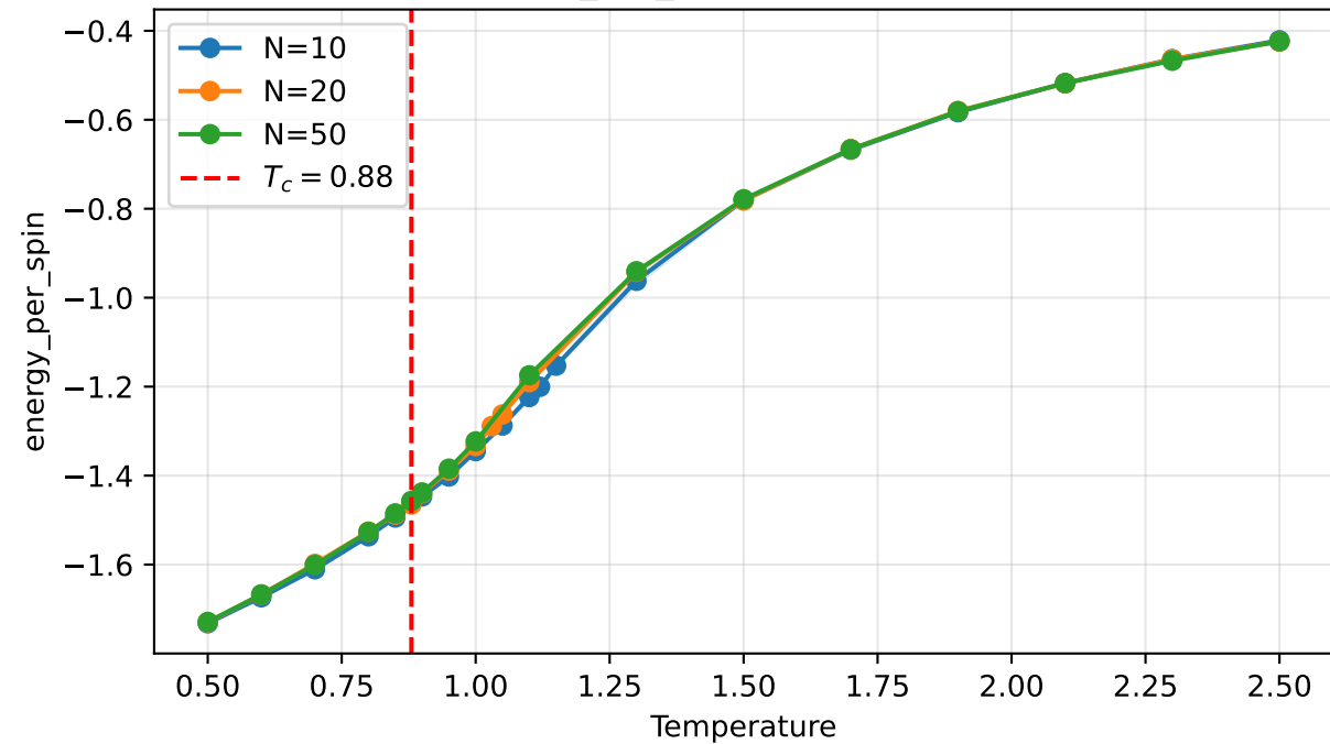
energy_per_spin vs temperature
