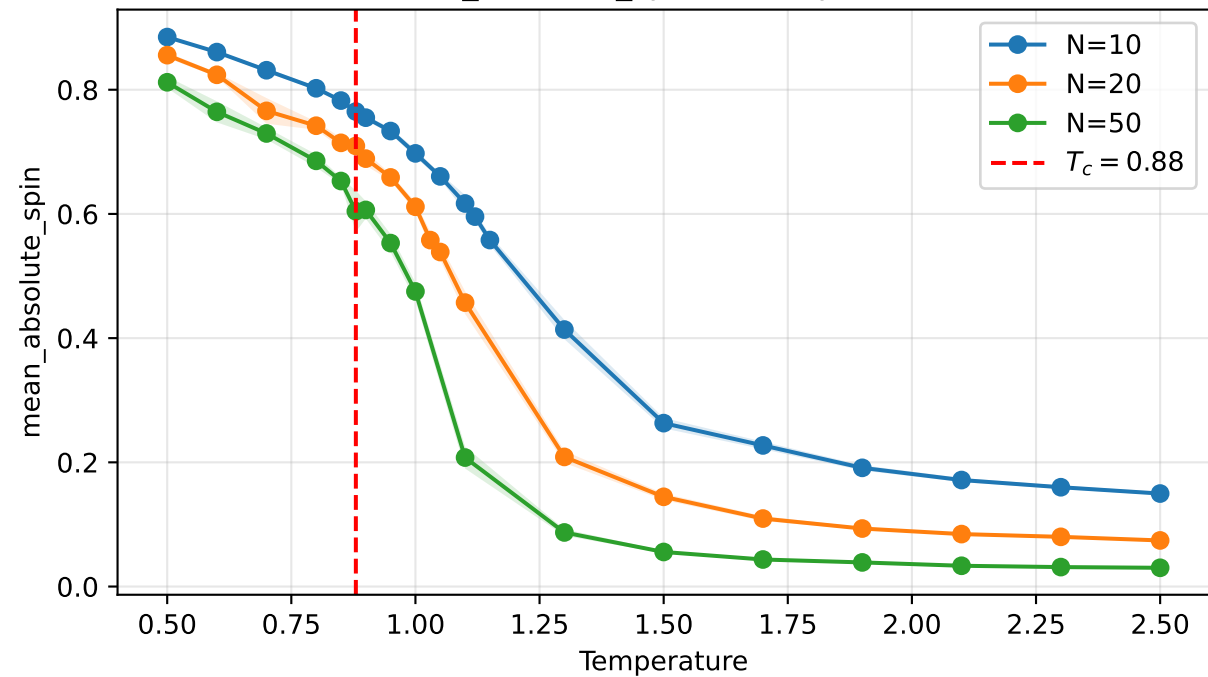
mean_absolute_spin vs temperature
