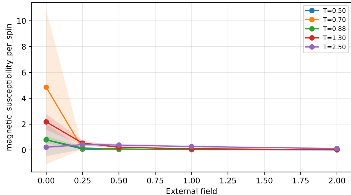
magnetic_susceptibility_per_spin vs external field, N=20
