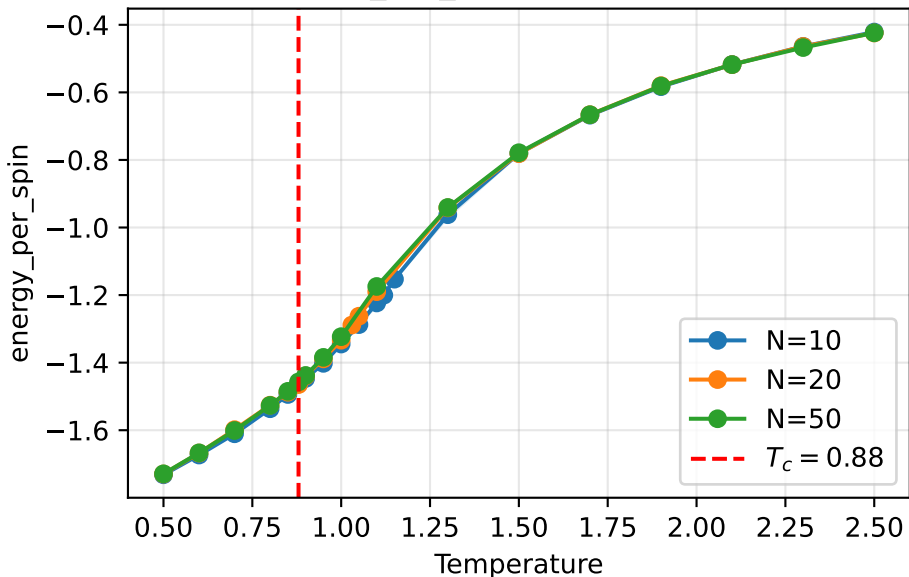
energy_per_spin vs temperature
