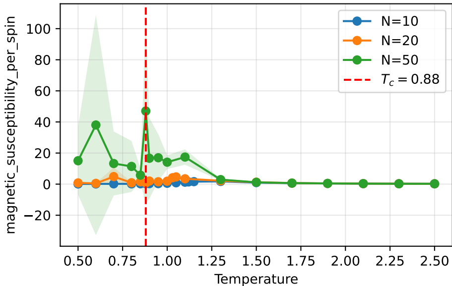
magnetic_susceptibility_per_spin vs temperature
