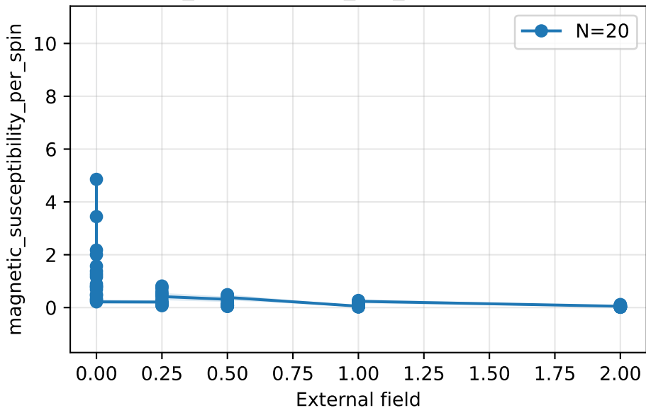
magnetic_susceptibility_per_spin vs external field
