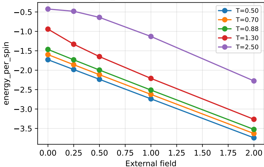
energy_per_spin vs external field, N=20
