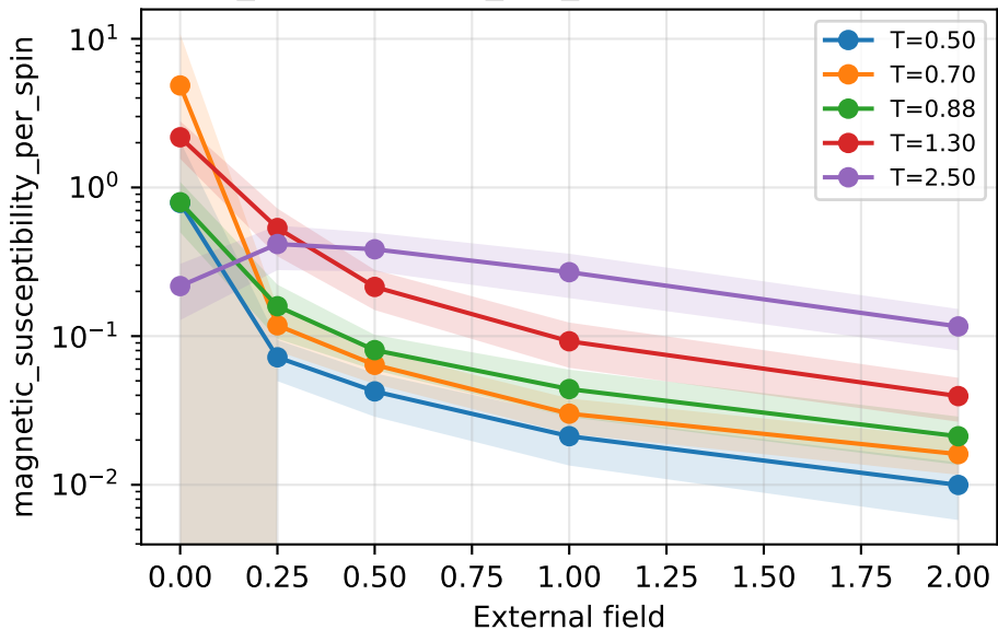
magnetic_susceptibility_per_spin vs external field, N=20
