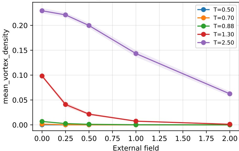
mean_vortex_density vs external field, N=20
