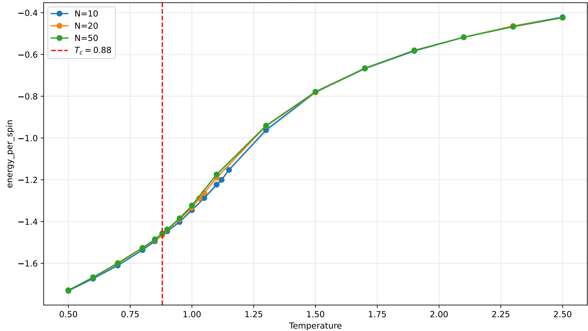
energy_per_spin vs temperature
