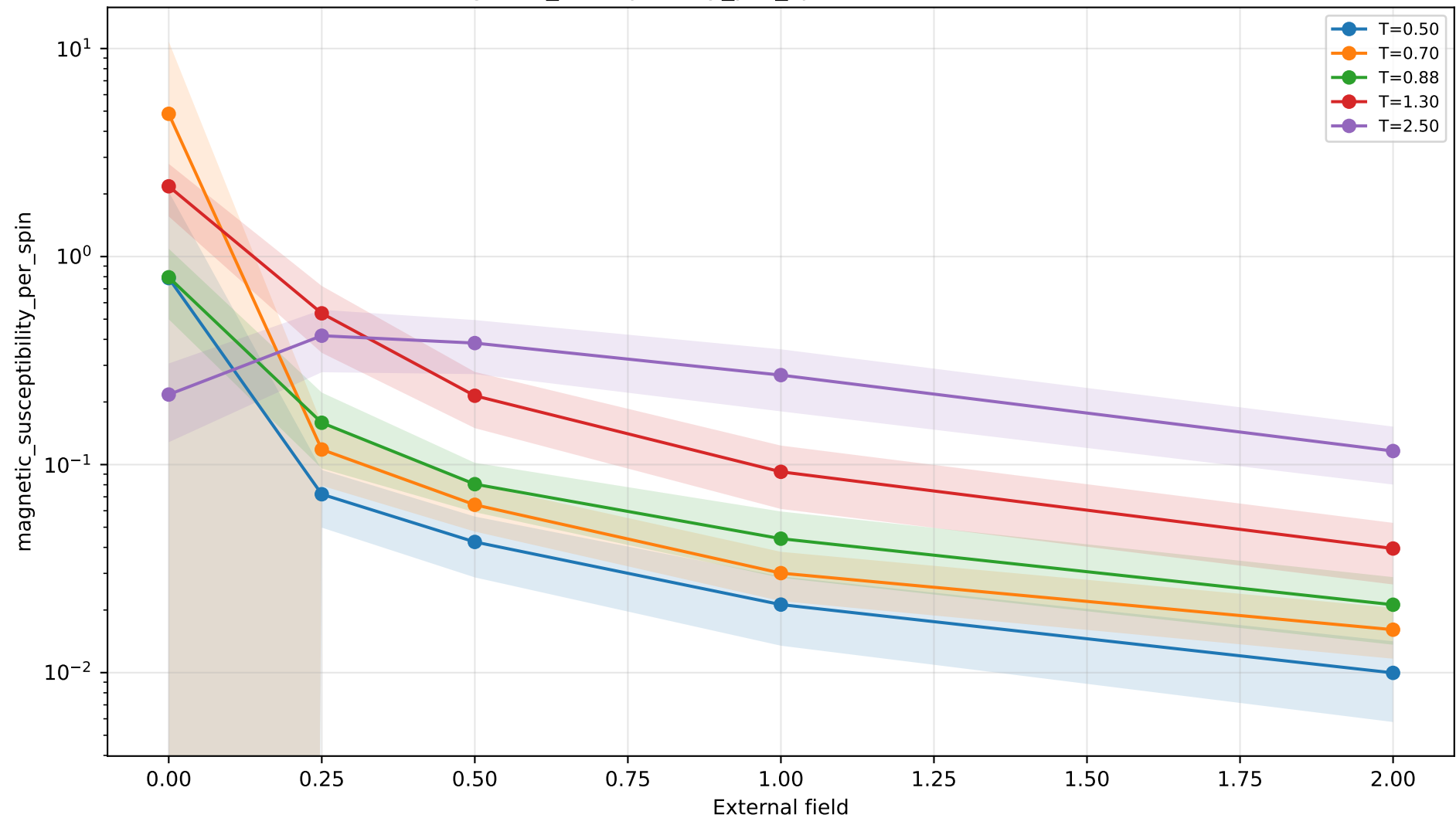
magnetic_susceptibility_per_spin vs external field, N=20
