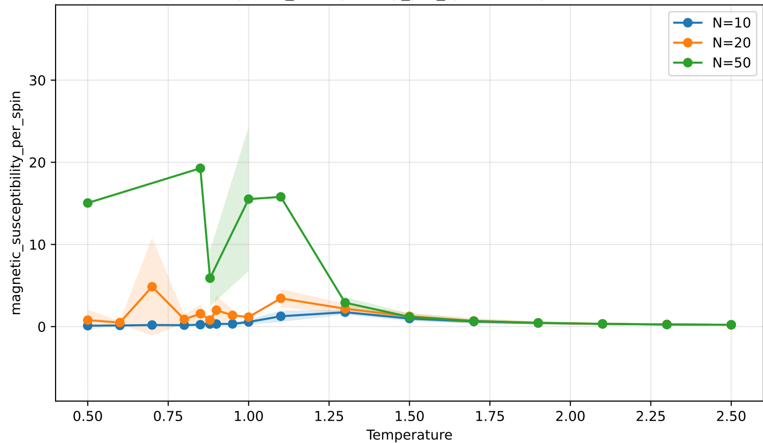
magnetic_susceptibility_per_spin vs temperature
