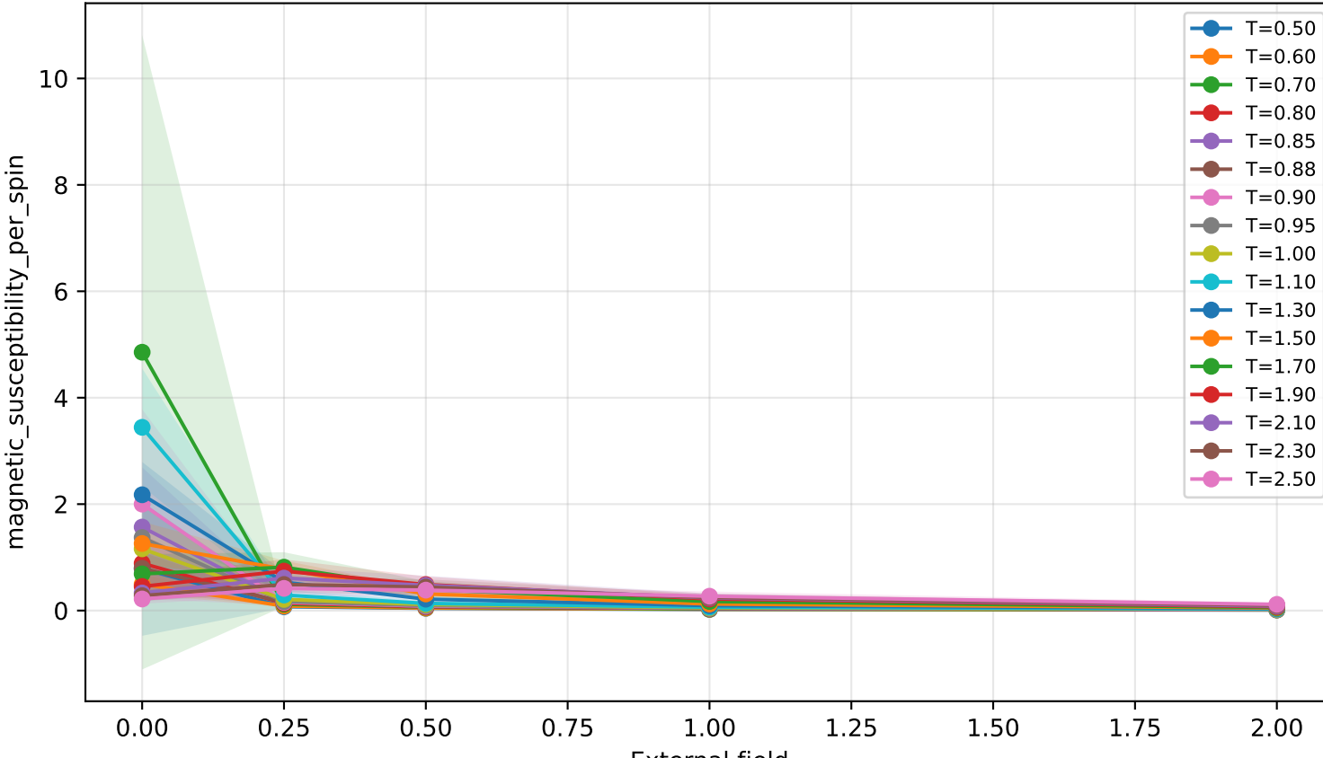
magnetic susceptibility per spin vs external field, N=20
