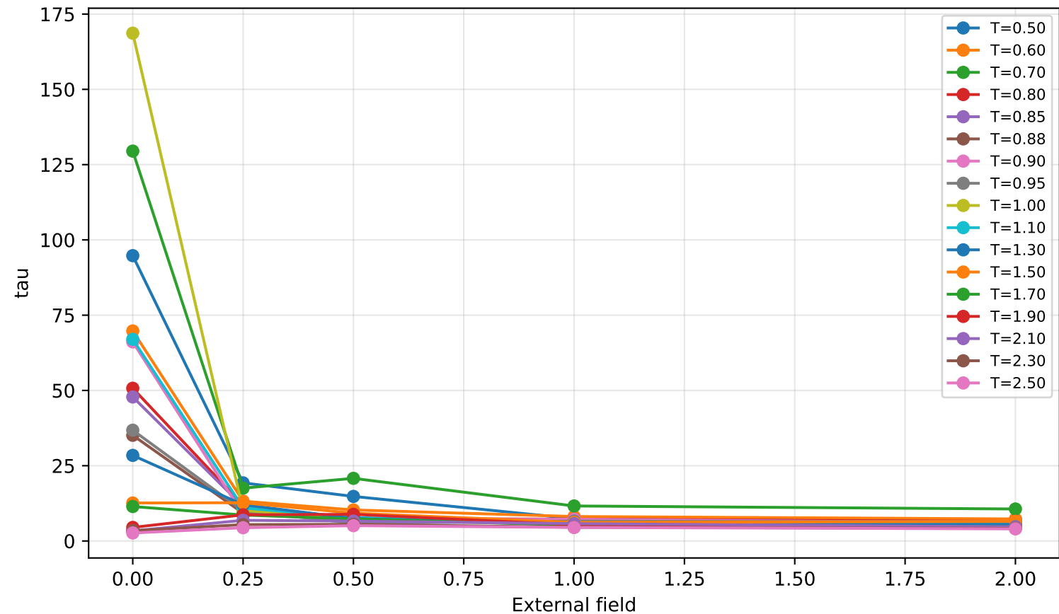
tau vs external field, N=20
