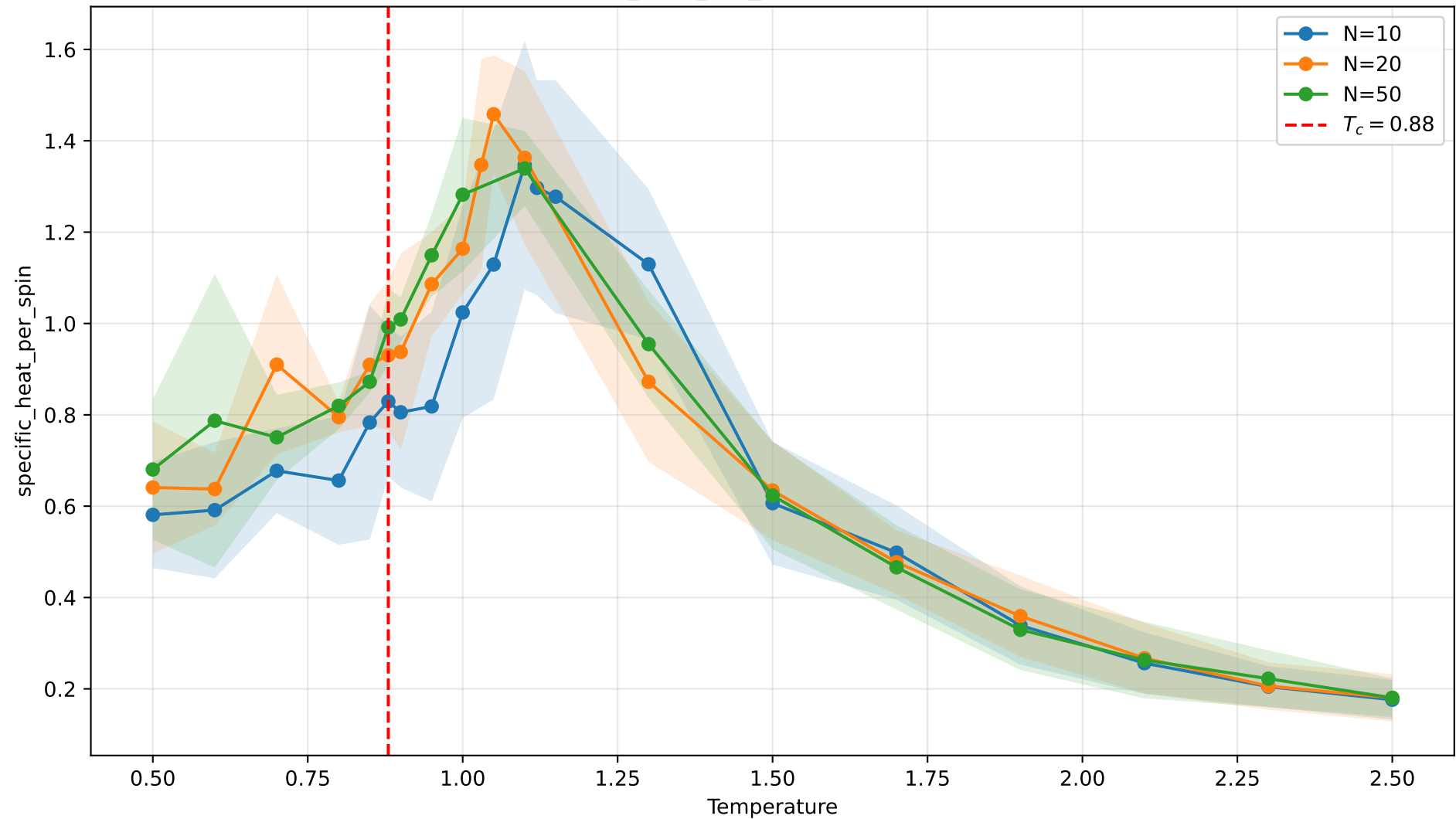
specific_heat_per_spin vs temperature
