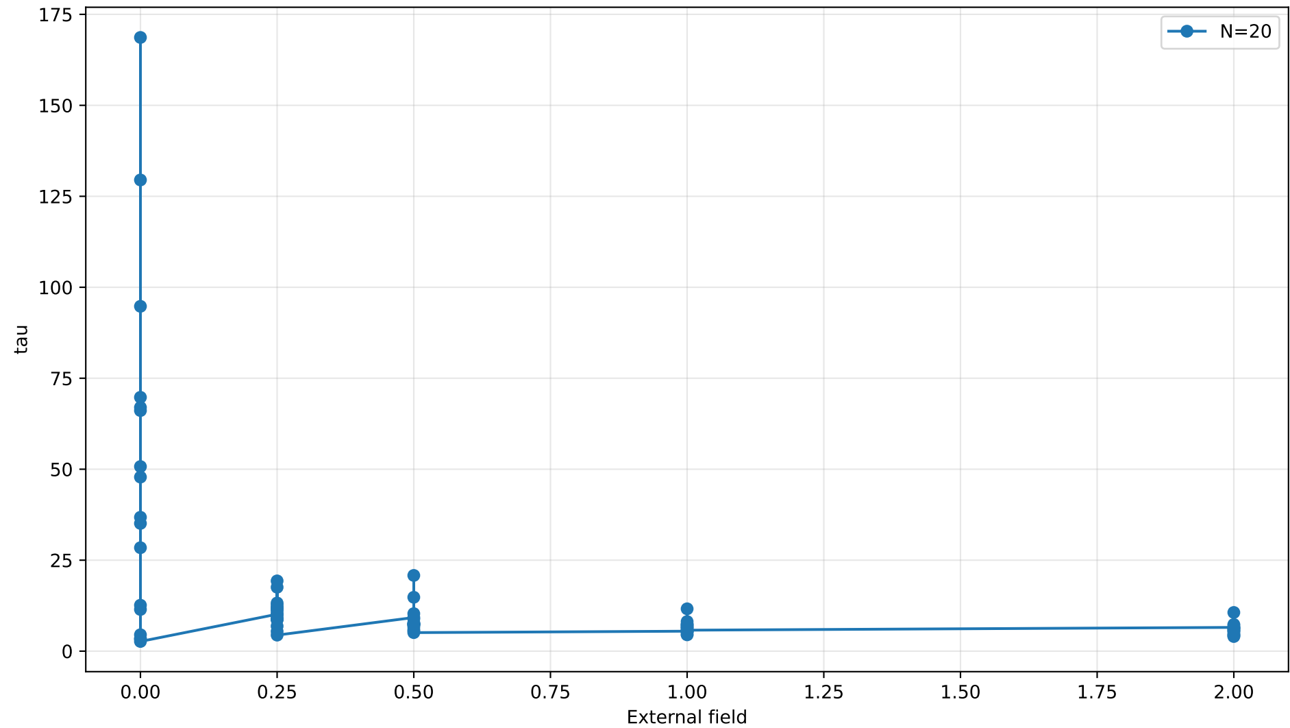
tau vs external field
