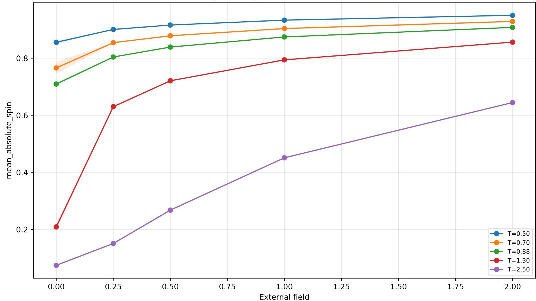
mean_absolute_spin vs external field, N=20
