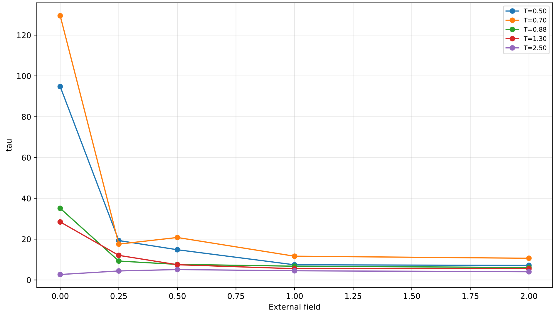
tau vs external field, N=20
