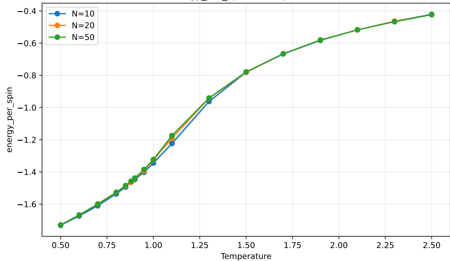
energy_per_spin vs temperature
