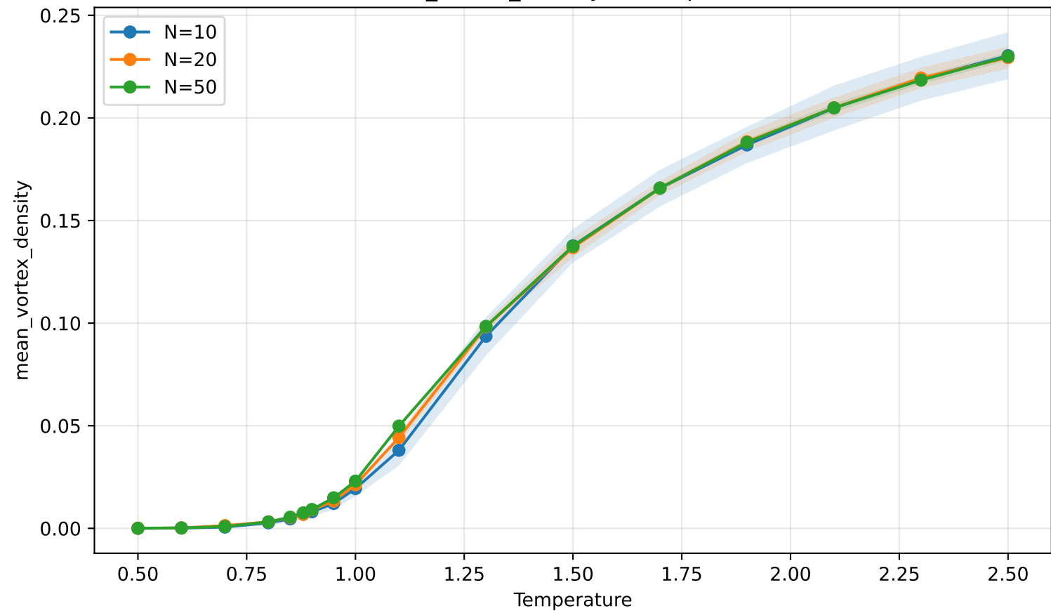
mean_vortex_density vs temperature
