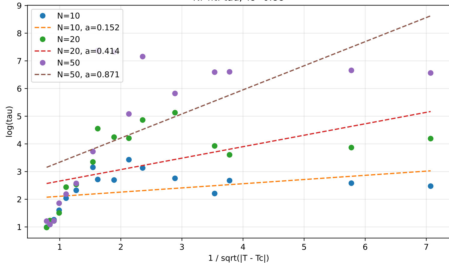
KT fit: tau, T_c=0.88
