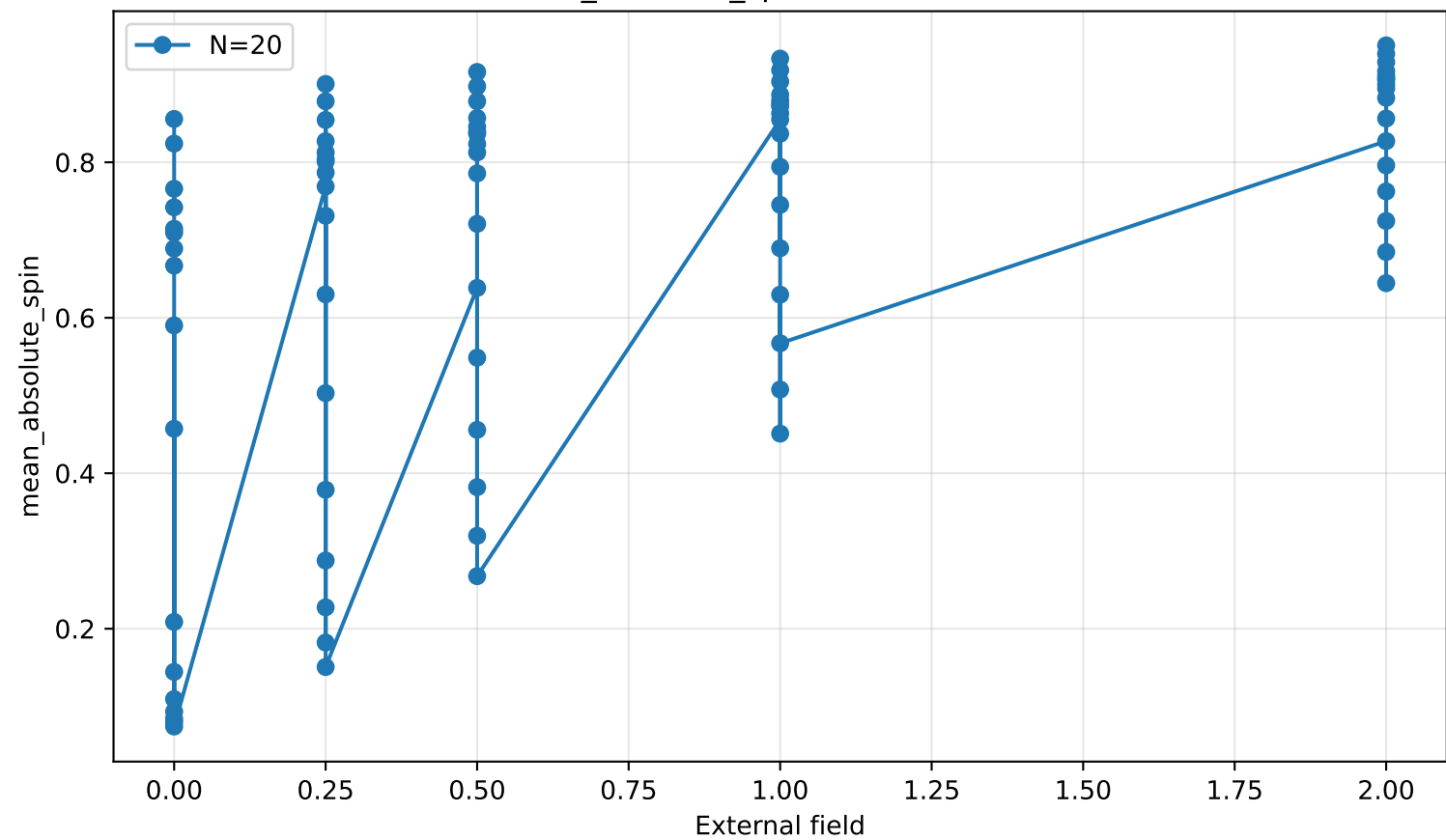
mean_absolute_spin vs external field
