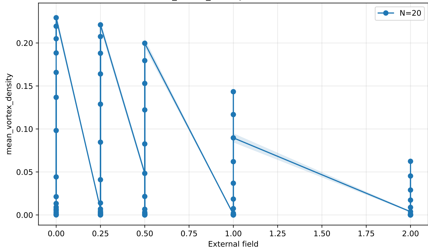
mean_vortex_density vs external field
