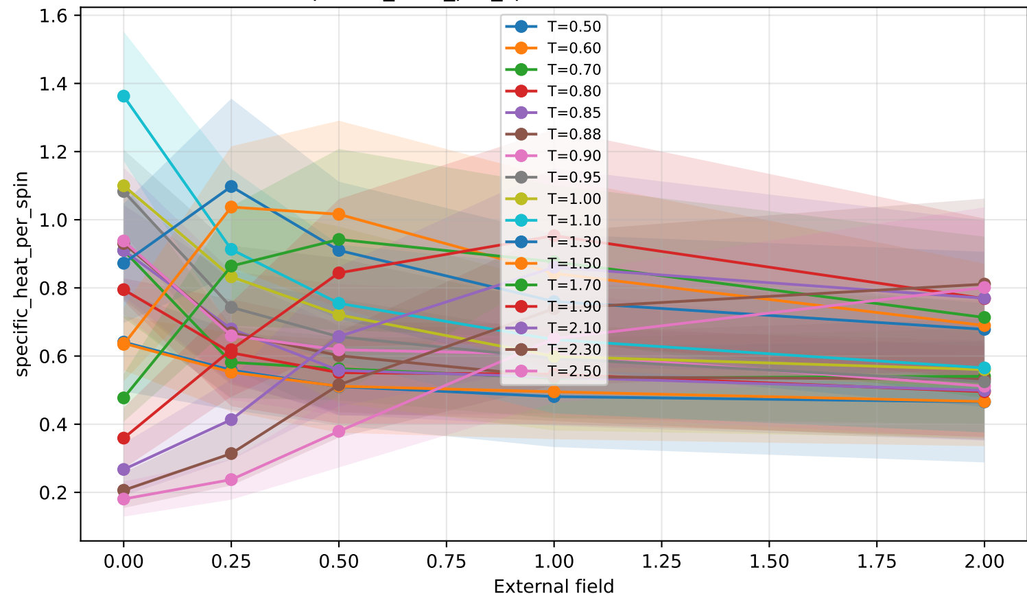
specific_heat_per_spin vs external field, N=20
