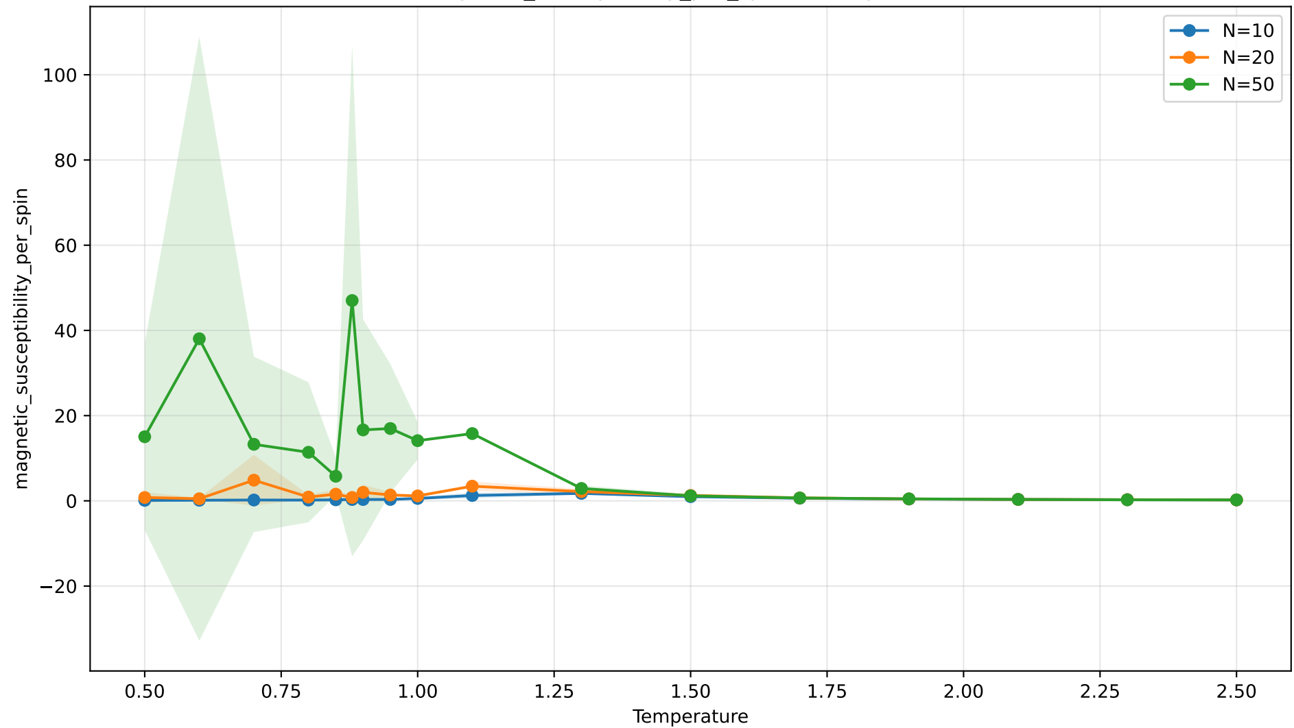
magnetic_susceptibility_per_spin vs temperature
