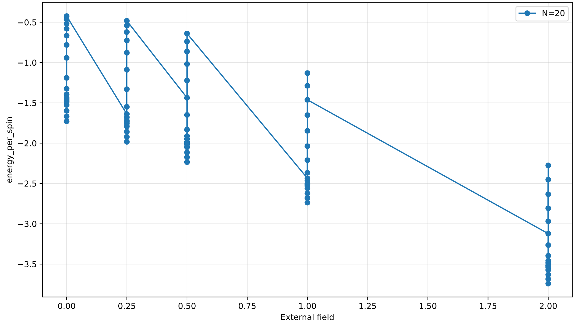
energy_per_spin vs external field
