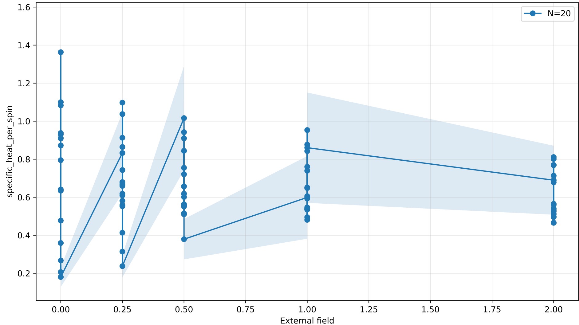
specific_heat_per_spin vs external field
