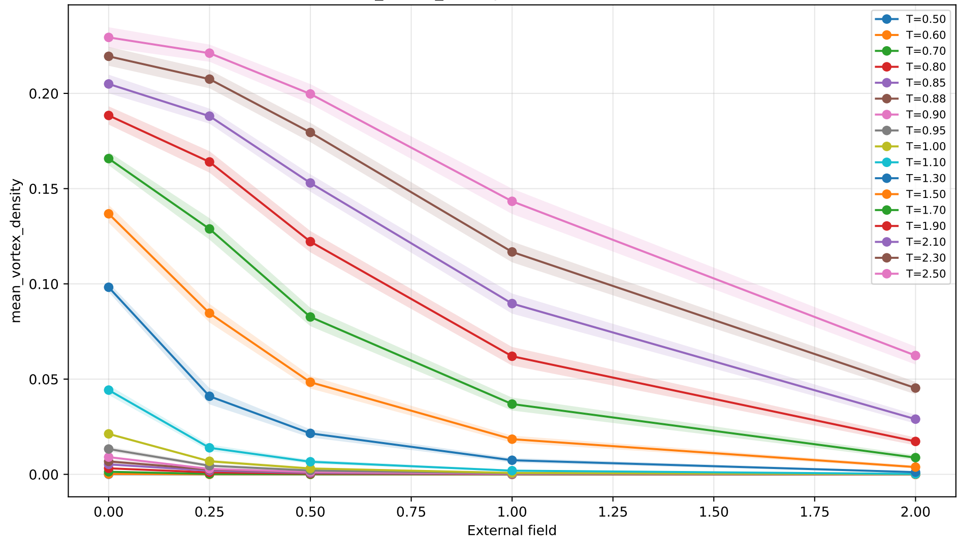
mean_vortex_density vs external field, N=20
