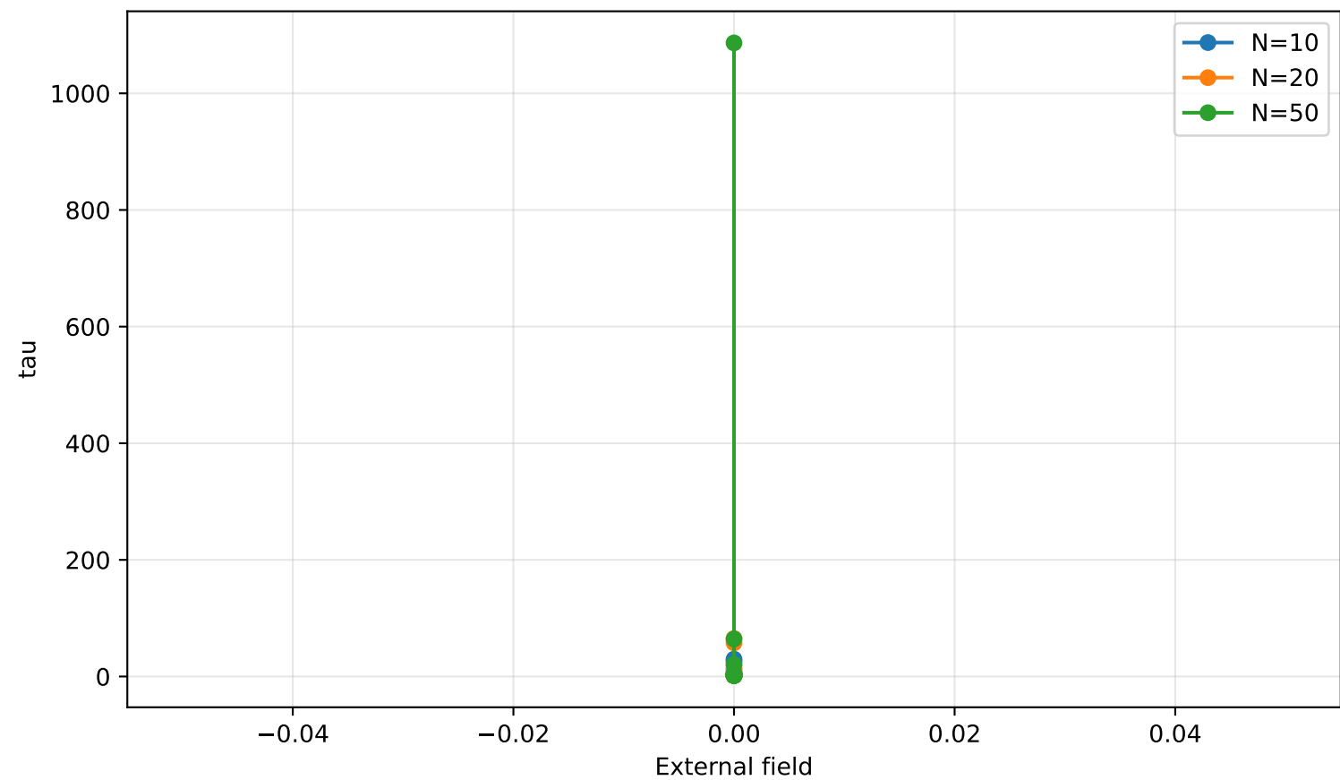
tau vs external field
