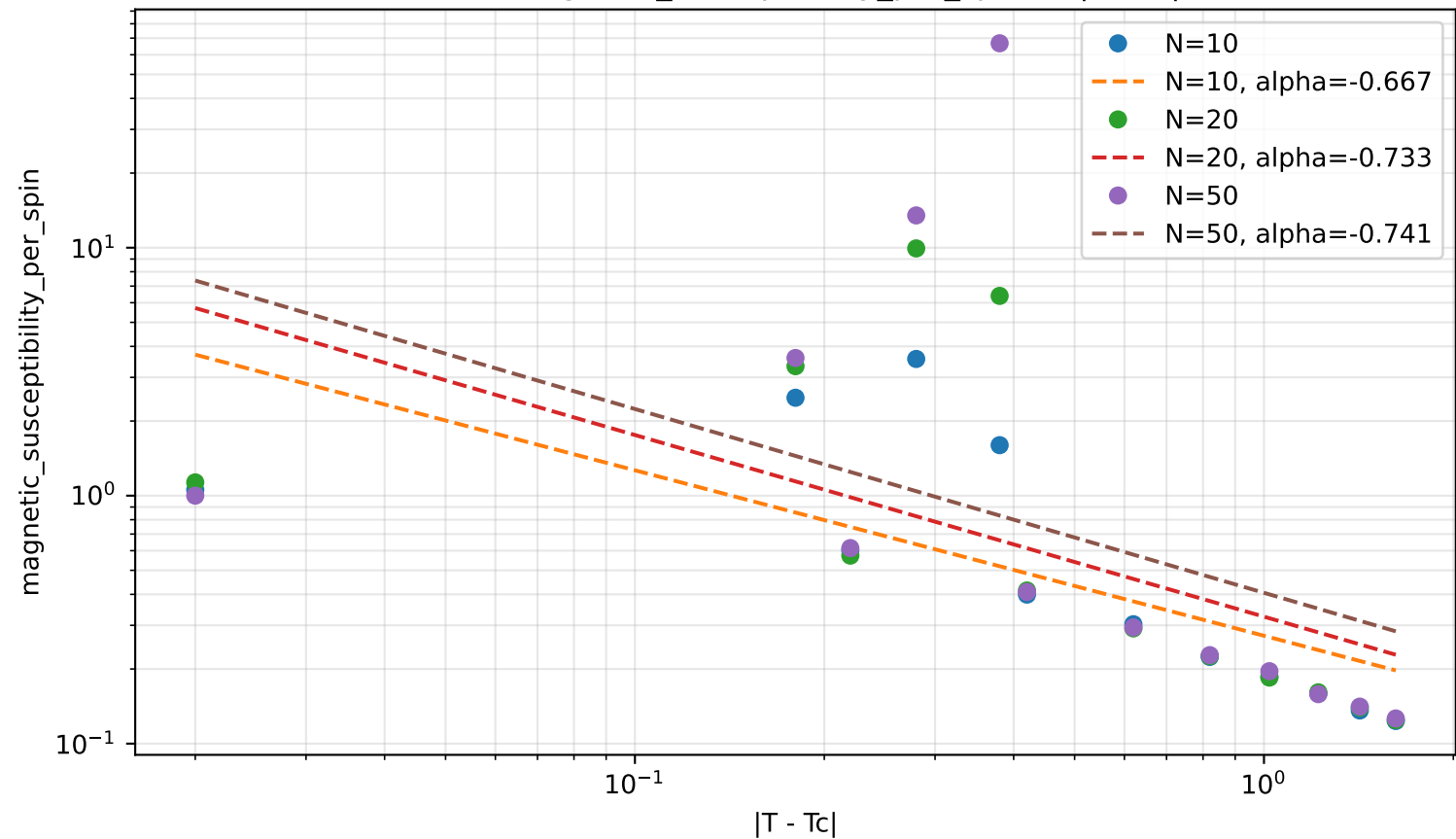
Power-law test: magnetic_susceptibility_per_spin vs |T - T_c| , T_c=0.88
