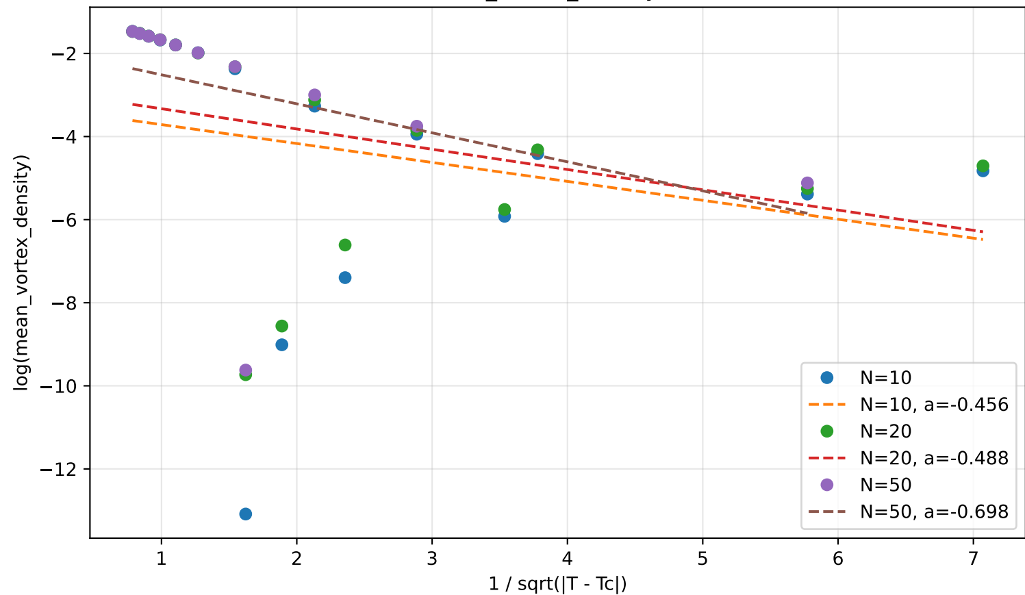
KT fit: mean_vortex_density, T_c=0.88
